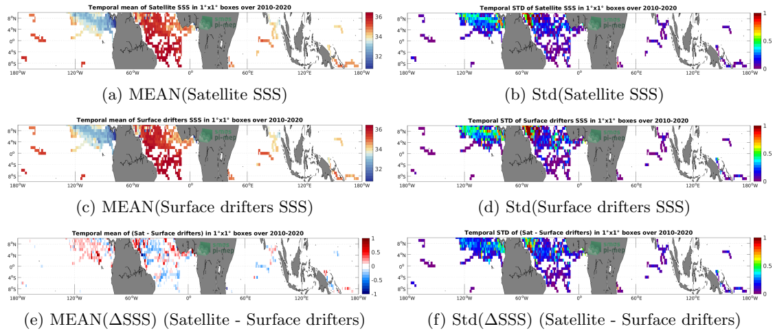
Figure 5: Temporal mean (left) and Std (right) of SSS from CCI SSS L4 Merged-OI v3.2 - 7-day running (ESA) (top), Surface drifters (middle), and of \Delta SSS (Satellite - Surface drifters). Only match-up pairs are used to generate these maps.
