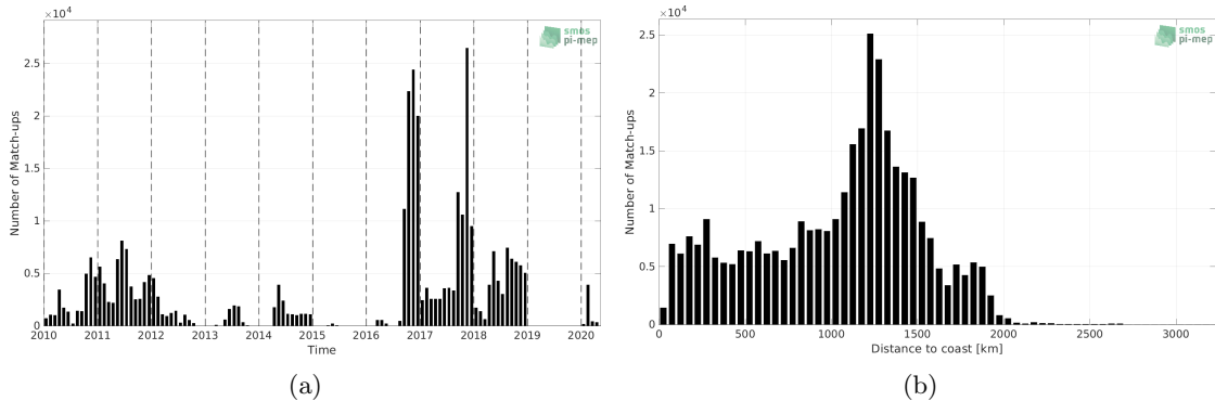
Figure 1: Number of match-ups between Surface drifters and CCI SSS L4 Merged-OI v3.2 - 7-day running (ESA) SSS as a function of time (a) and as function of the distance to coast (b) over the Equatorial Ocean 10N-10S Pi-MEP region and for the full satellite product period.
