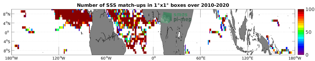
Figure 3: Number of SSS match-ups between Surface drifters SSS and the CCI SSS L4 Merged-OI v3.2 - 7-day running (ESA) SSS product for the Equatorial Ocean 10N-10S Pi-MEP region over 1^\circ \times 1^\circ boxes and for the full satellite product period.
