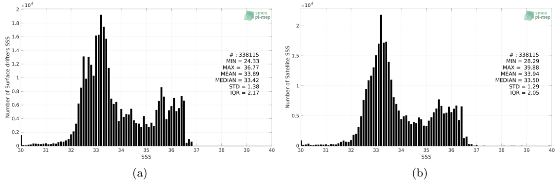
Figure 2: Histograms of SSS from Surface drifters (a) and CCI SSS L4 Merged-OI v3.2 - 7-day running (ESA) (b) considering all match-up pairs per bins of 0.1 over the Equatorial Ocean 10N-10S Pi-MEP region and for the full satellite product period.
