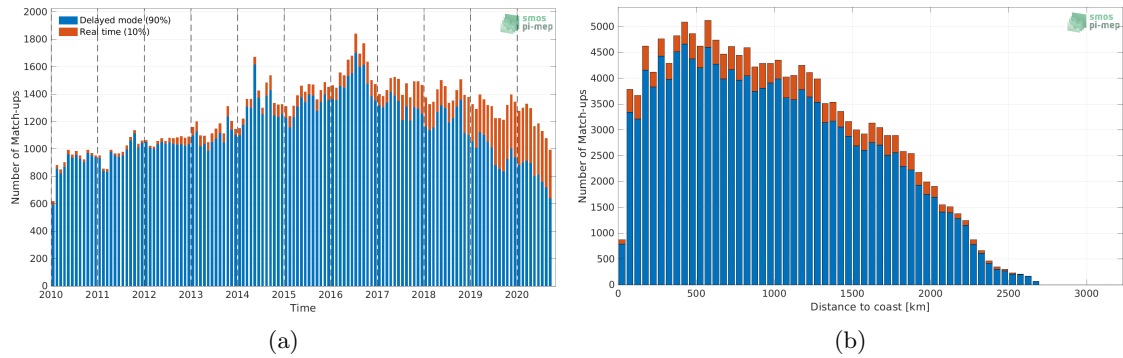
Figure 1: Number of match-ups between Argo and CCI SSS L4 Merged-OI v3.2 - 7-day running (ESA) SSS as a function of time (a) and as function of the distance to coast (b) over the Equatorial Ocean 10N-10S Pi-MEP region and for the full satellite product period.
