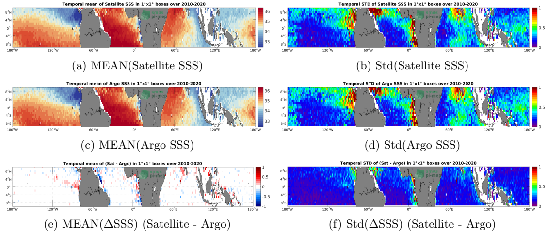
Figure 6: Temporal mean (left) and Std (right) of SSS from CCI SSS L4 Merged-OI v3.2 - 7-day running (ESA) (top), Argo (middle), and of \Delta SSS (Satellite - Argo). Only match-up pairs are used to generate these maps.
