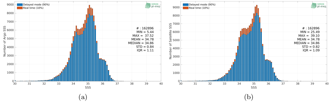
Figure 2: Histograms of SSS from Argo (a) and CCI SSS L4 Merged-OI v3.2 - 7-day running (ESA) (b) considering all match-up pairs per bins of 0.1 over the Equatorial Ocean 10N-10S Pi-MEP region and for the full satellite product period.
