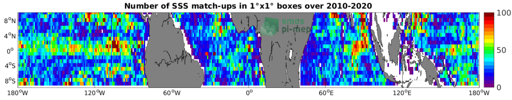
Figure 4: Number of SSS match-ups between Argo SSS and the CCI SSS L4 Merged-OI v3.2 - 7-day running (ESA) SSS product for the Equatorial Ocean 10N-10S Pi-MEP region over 1^\circ \times 1^\circ boxes and for the full satellite product period.
