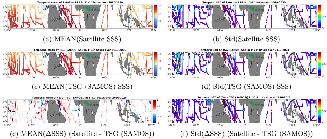
Figure 6: Temporal mean (left) and Std (right) of SSS from CCI SSS L4 Merged-OI v3.2 - 30-day running (ESA) (top), TSG (SAMOS) (middle), and of \Delta SSS (Satellite - TSG (SAMOS)). Only match-up pairs are used to generate these maps.
