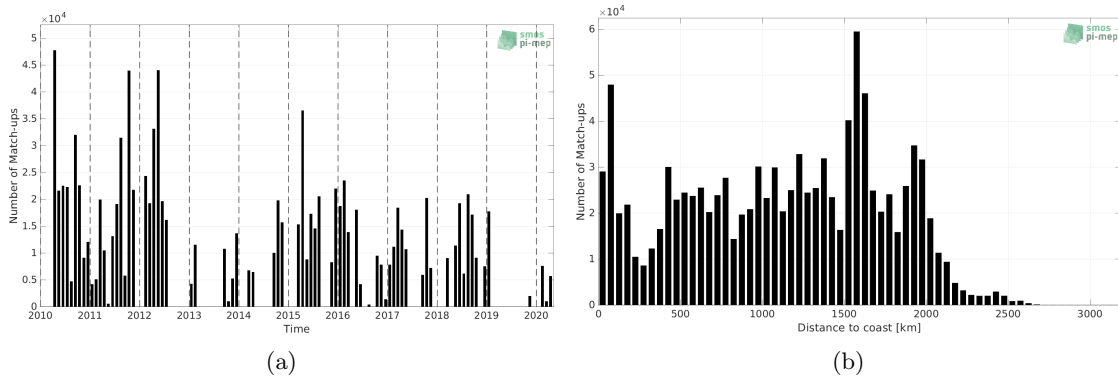
Figure 1: Number of match-ups between TSG (SAMOS) and CCI SSS L4 Merged-OI v3.2 - 30-day running (ESA) SSS as a function of time (a) and as function of the distance to coast (b) over the Equatorial Ocean 10N-10S Pi-MEP region and for the full satellite product period.
