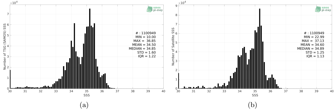
Figure 2: Histograms of SSS from TSG (SAMOS) (a) and CCI SSS L4 Merged-OI v3.2 - 30-day running (ESA) (b) considering all match-up pairs per bins of 0.1 over the Equatorial Ocean 10N-10S Pi-MEP region and for the full satellite product period.
