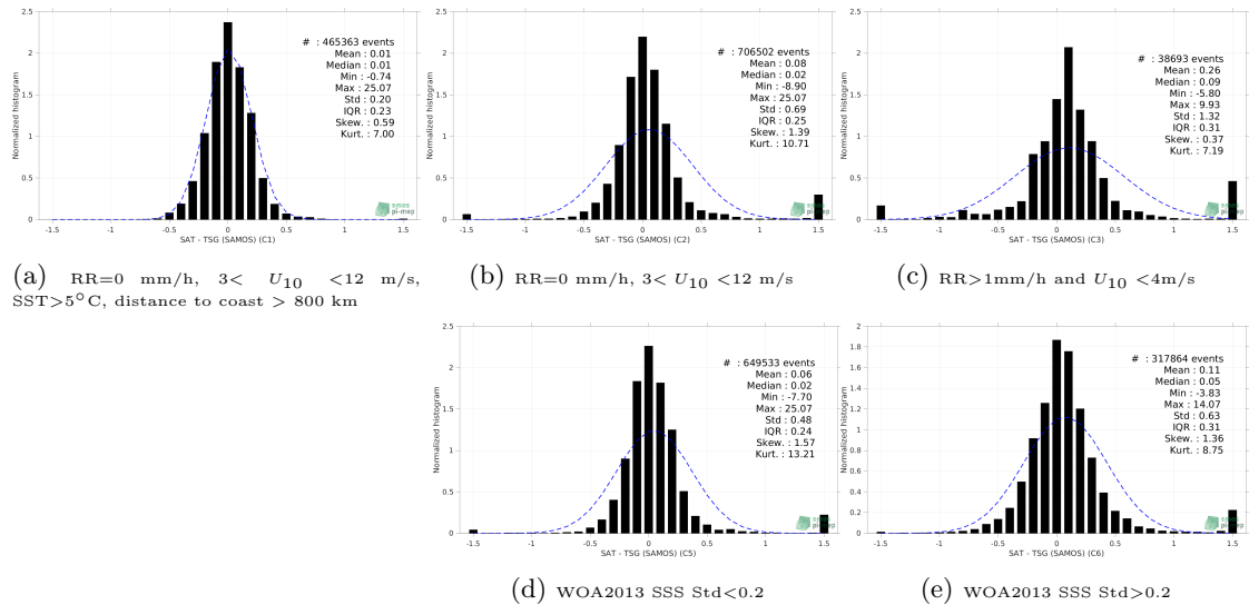
Figure 13: Normalized histogram of \Delta SSS (CCI SSS L4 Merged-OI v3.2 - 30-day running (ESA) - TSG (SAMOS)) for 5 different subdatasets corresponding to: RR=0 mm/h, 3 < U_{10} < 12 m/s, SST >5^\circ\text{C} , distance to coast > 800 km (a), RR=0 mm/h, 3 < U_{10} < 12 m/s (b), RR >1 mm/h and U_{10} < 4 m/s (c), WOA2013 SSS Std <0.2 (d), WOA2013 SSS Std >0.2 (e).
