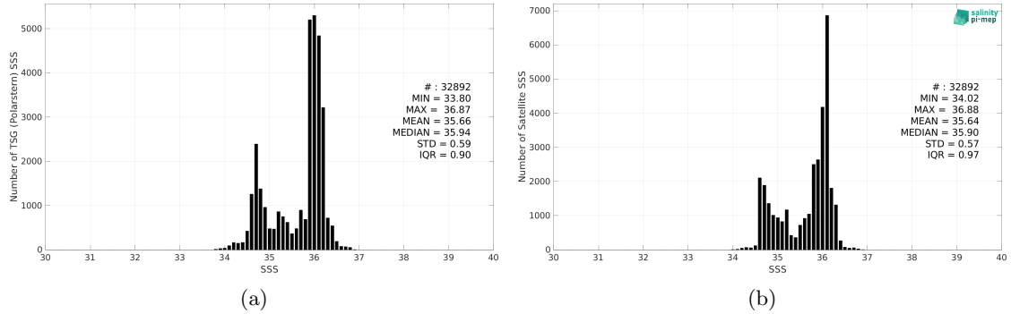
Figure 2: Histograms of SSS from TSG (Polarstern) (a) and CCI SSS L4 Merged-OI v3.2 - 30-day running (ESA) (b) considering all match-up pairs per bins of 0.1 over the Equatorial Ocean 10N-10S Pi-MEP region and for the full satellite product period.
