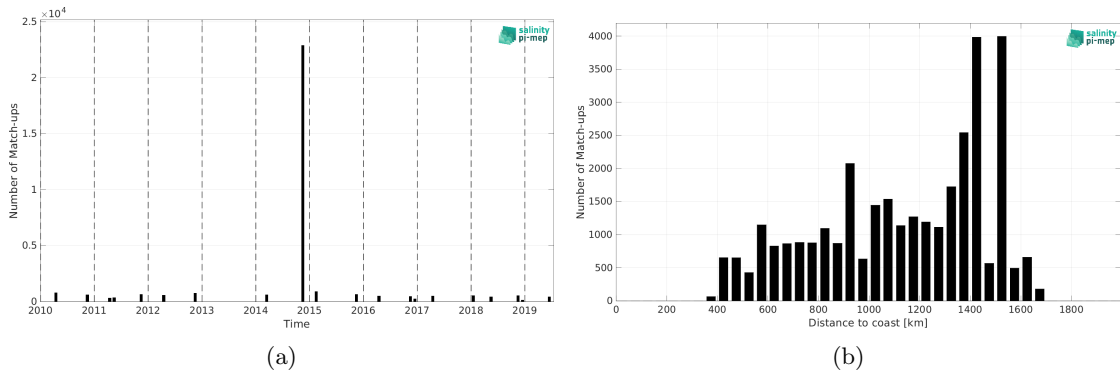
Figure 1: Number of match-ups between TSG (Polarstern) and CCI SSS L4 Merged-OI v3.2 - 30-day running (ESA) SSS as a function of time (a) and as function of the distance to coast (b) over the Equatorial Ocean 10N-10S Pi-MEP region and for the full satellite product period.
