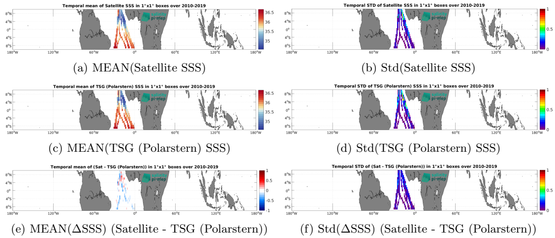
Figure 6: Temporal mean (left) and Std (right) of SSS from CCI SSS L4 Merged-OI v3.2 - 30-day running (ESA) (top), TSG (Polarstern) (middle), and of \Delta SSS (Satellite - TSG (Polarstern)). Only match-up pairs are used to generate these maps.
