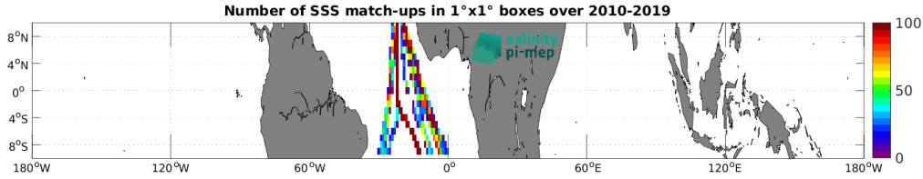
Figure 4: Number of SSS match-ups between TSG (Polarstern) SSS and the CCI SSS L4 Merged-OI v3.2 - 30-day running (ESA) SSS product for the Equatorial Ocean 10N-10S Pi-MEP region over 1^\circ \times 1^\circ boxes and for the full satellite product period.
