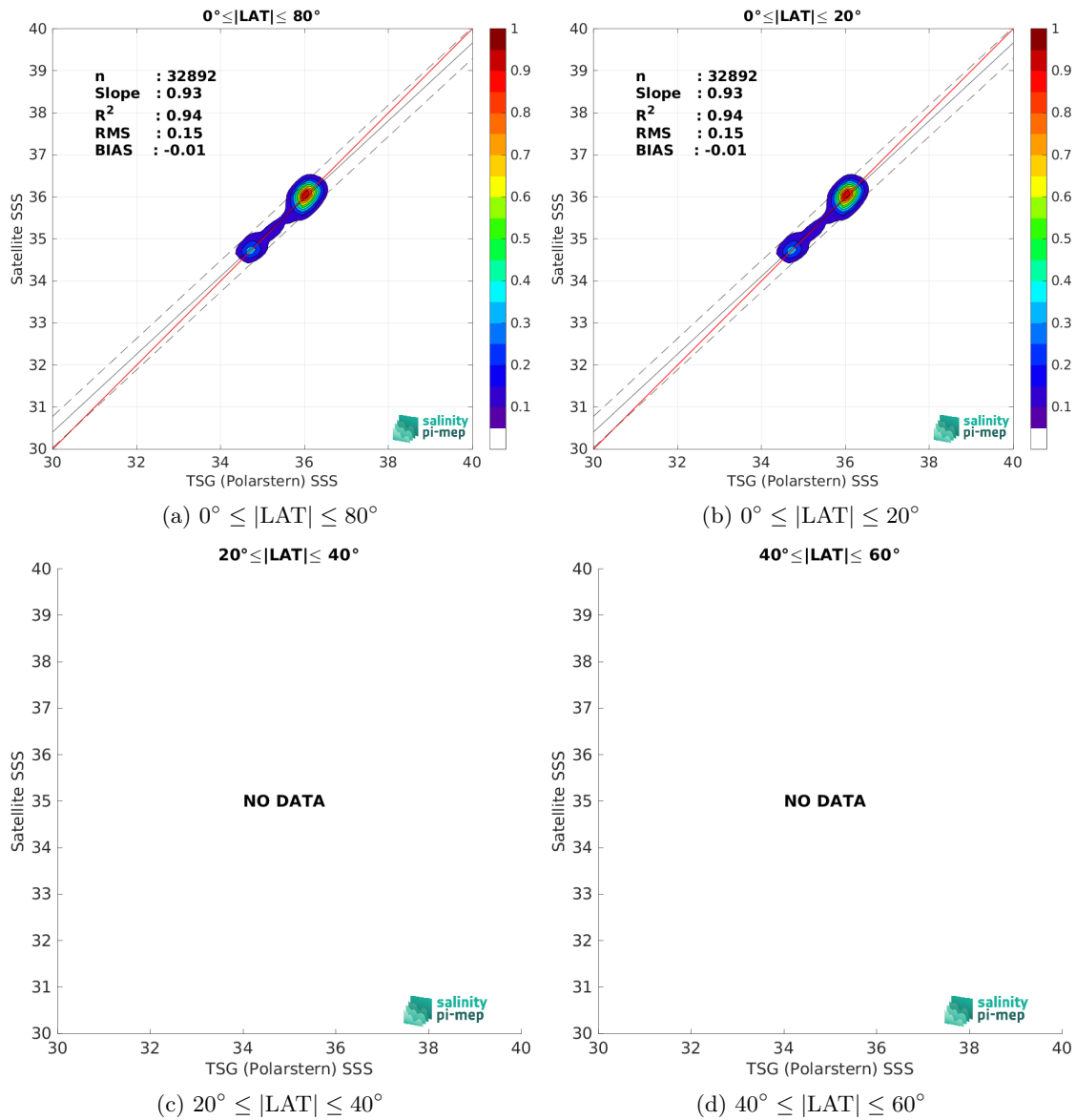
Figure 9: Contour maps of the concentration of CCI SSS L4 Merged-OI v3.2 - 30-day running (ESA) SSS ( y -axis) versus TSG (Polarstern) SSS ( x -axis) at match-up pairs for different latitude bands. For each plot, the red line shows x=y . The black thin and dashed lines indicate a linear fit through the data cloud and the \pm 95\% confidence levels, respectively. The number match-up pairs n , the slope and R^2 coefficient of the linear fit, the root mean square (RMS) and the mean bias between satellite and in situ data are indicated for each latitude band in each plots.
