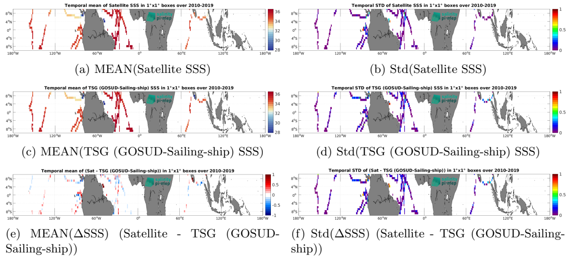
Figure 6: Temporal mean (left) and Std (right) of SSS from CCI SSS L4 Merged-OI v3.2 - 30-day running (ESA) (top), TSG (GOSUD-Sailing-ship) (middle), and of \Delta SSS (Satellite - TSG (GOSUD-Sailing-ship)). Only match-up pairs are used to generate these maps.
