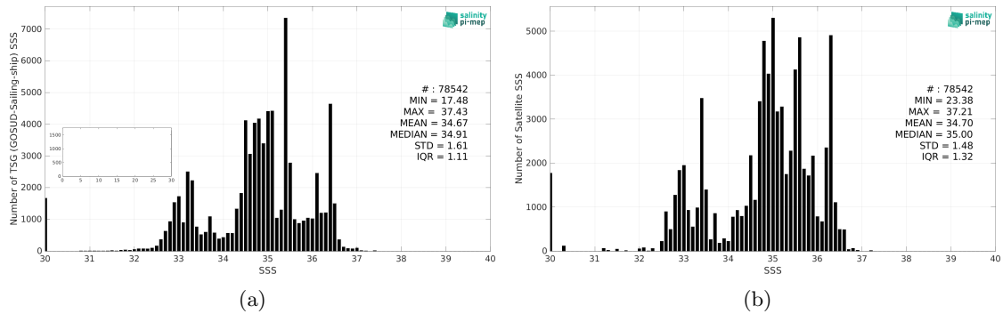
Figure 2: Histograms of SSS from TSG (GOSUD-Sailing-ship) (a) and CCI SSS L4 Merged-OI v3.2 - 30-day running (ESA) (b) considering all match-up pairs per bins of 0.1 over the Equatorial Ocean 10N-10S Pi-MEP region and for the full satellite product period.
