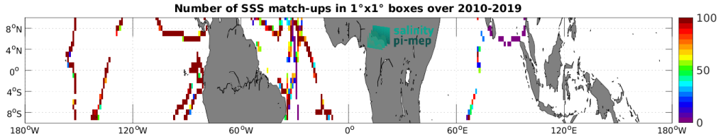
Figure 4: Number of SSS match-ups between TSG (GOSUD-Sailing-ship) SSS and the CCI SSS L4 Merged-OI v3.2 - 30-day running (ESA) SSS product for the Equatorial Ocean 10N-10S Pi-MEP region over 1^\circ \times 1^\circ boxes and for the full satellite product period.
