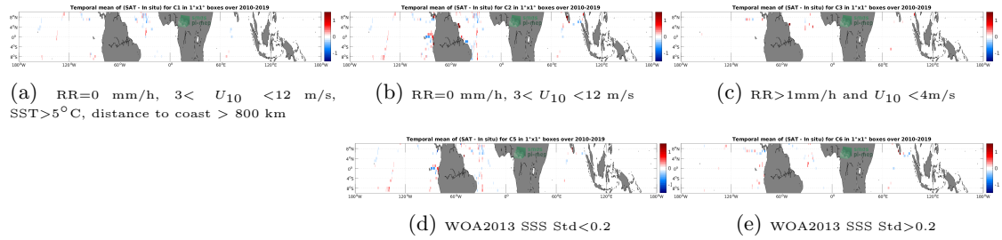
Figure 12: Temporal mean gridded over spatial boxes of size 1^\circ \times 1^\circ of \Delta SSS (CCI SSS L4 Merged-OI v3.2 - 30-day running (ESA) - TSG (GOSUD-Sailing-ship)) for 5 different subdatasets corresponding to:RR=0 mm/h, 3 < U_{10} < 12 m/s, SST >5^\circ\text{C} , distance to coast > 800 km (a), RR=0 mm/h, 3 < U_{10} < 12 m/s (b), RR >1 mm/h and U_{10} < 4 m/s (c), WOA2013 SSS Std <0.2 (d), WOA2013 SSS Std >0.2 (e).
