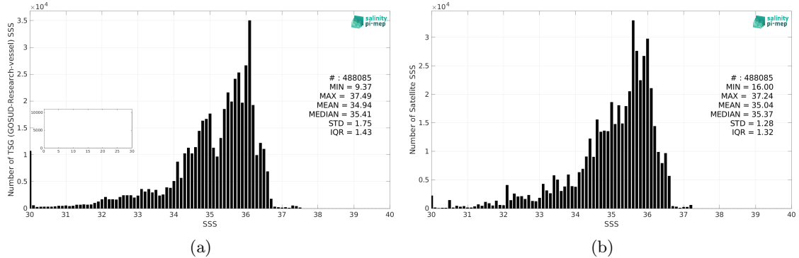
Figure 2: Histograms of SSS from TSG (GOSUD-Research-vessel) (a) and CCI SSS L4 Merged-OI v3.2 - 30-day running (ESA) (b) considering all match-up pairs per bins of 0.1 over the Equatorial Ocean 10N-10S Pi-MEP region and for the full satellite product period.
