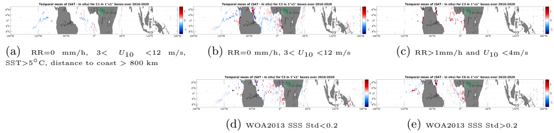
Figure 12: Temporal mean gridded over spatial boxes of size 1^{\circ}\times 1^{\circ} of \Delta SSS (CCI SSS L4 Merged-OI v3.2 - 30-day running (ESA) - TSG (GOSUD-Research-vessel)) for 5 different subdatasets corresponding to:RR=0 mm/h, 3 < U_{10} < 12 m/s, SST >5^{\circ}\text{C} , distance to coast > 800 km (a), RR=0 mm/h, 3 < U_{10} < 12 m/s (b), RR >1 mm/h and U_{10} < 4 m/s (c), WOA2013 SSS Std <0.2 (d), WOA2013 SSS Std >0.2 (e).
