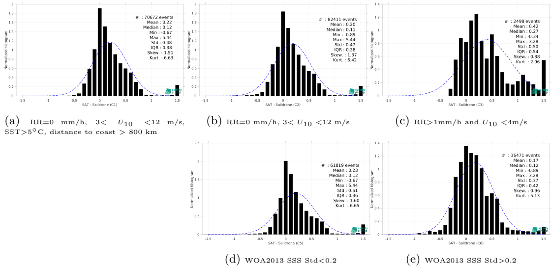
Figure 13: Normalized histogram of \Delta\text{SSS} (CCI SSS L4 Merged-OI v3.2 - 30-day running (ESA) - Saildrone) for 5 different subdatasets corresponding to: RR=0 mm/h, 3 < U_{10} < 12 m/s, SST >5^\circ\text{C} , distance to coast > 800 km (a), RR=0 mm/h, 3 < U_{10} < 12 m/s (b), RR >1 mm/h and U_{10} < 4 m/s (c), WOA2013 SSS Std <0.2 (d), WOA2013 SSS Std >0.2 (e).
