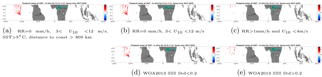
Figure 12: Temporal mean gridded over spatial boxes of size 1^\circ \times 1^\circ of \Delta\text{SSS} (CCI SSS L4 Merged-OI v3.2 - 30-day running (ESA) - Saildrone) for 5 different subdatasets corresponding to: RR=0 mm/h, 3 < U_{10} < 12 m/s, SST >5^\circ\text{C} , distance to coast > 800 km (a), RR=0 mm/h, 3 < U_{10} < 12 m/s (b), RR >1 mm/h and U_{10} < 4 m/s (c), WOA2013 SSS Std <0.2 (d), WOA2013 SSS Std >0.2 (e).
