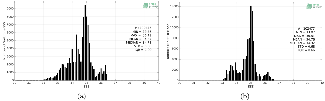
Figure 2: Histograms of SSS from Saildrone (a) and CCI SSS L4 Merged-OI v3.2 - 30-day running (ESA) (b) considering all match-up pairs per bins of 0.1 over the Equatorial Ocean 10N-10S Pi-MEP region and for the full satellite product period.
