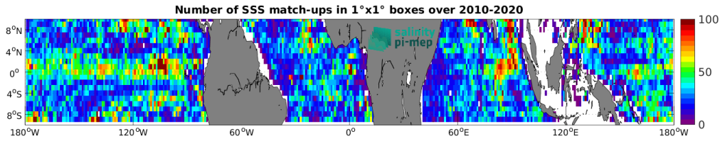
Figure 4: Number of SSS match-ups between Argo SSS and the CCI SSS L4 Merged-OI v3.2 - 30-day running (ESA) SSS product for the Equatorial Ocean 10N-10S Pi-MEP region over 1^\circ \times 1^\circ boxes and for the full satellite product period.
