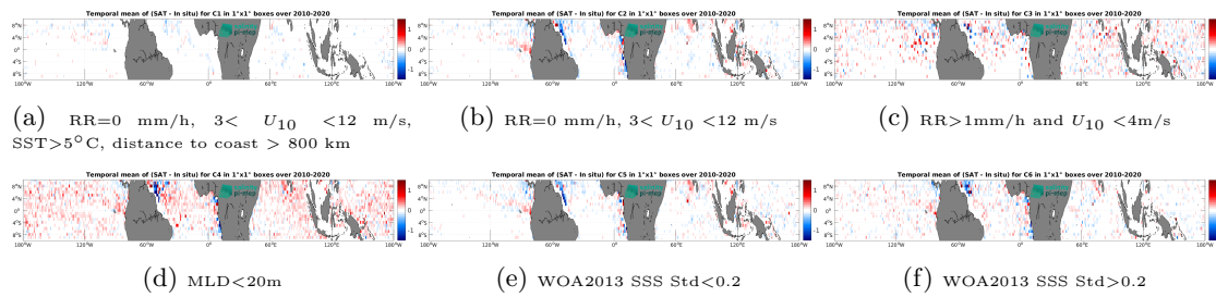
Figure 12: Temporal mean gridded over spatial boxes of size 1^\circ \times 1^\circ of \Delta SSS (CCI SSS L4 Merged-OI v3.2 - 30-day running (ESA) - Argo) for 6 different subdatasets corresponding to:RR=0 mm/h, 3 < U_{10} < 12 m/s, SST >5^\circ C, distance to coast > 800 km (a), RR=0 mm/h, 3 < U_{10} < 12 m/s (b), RR >1 mm/h and U_{10} < 4 m/s (c),MLD <20 m (d),WOA2013 SSS Std <0.2 (e),WOA2013 SSS Std >0.2 (f).
