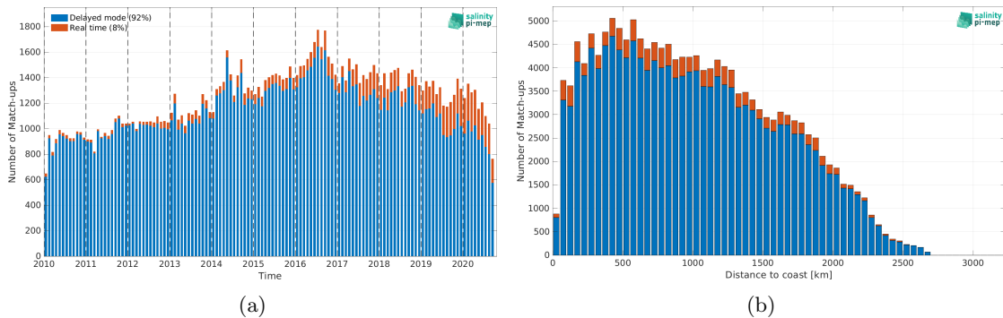
Figure 1: Number of match-ups between Argo and CCI SSS L4 Merged-OI v3.2 - 30-day running (ESA) SSS as a function of time (a) and as function of the distance to coast (b) over the Equatorial Ocean 10N-10S Pi-MEP region and for the full satellite product period.
