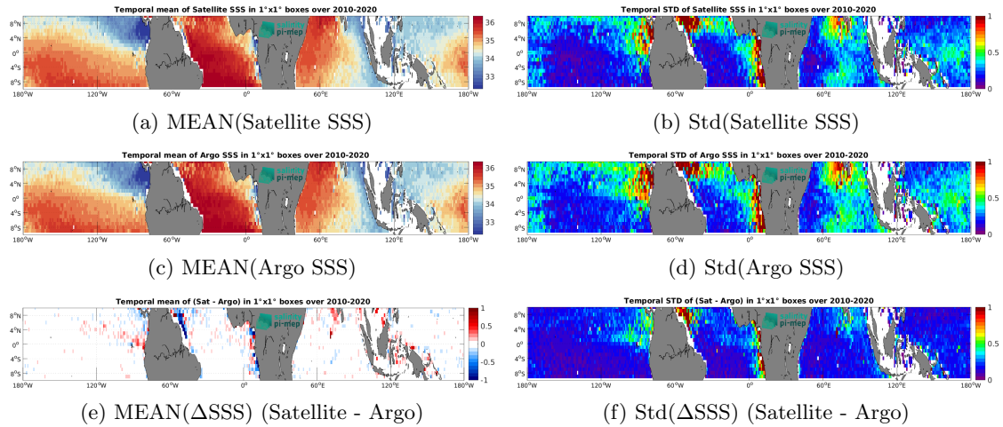
Figure 6: Temporal mean (left) and Std (right) of SSS from CCI SSS L4 Merged-OI v3.2 - 30-day running (ESA) (top), Argo (middle), and of \Delta SSS (Satellite - Argo). Only match-up pairs are used to generate these maps.
