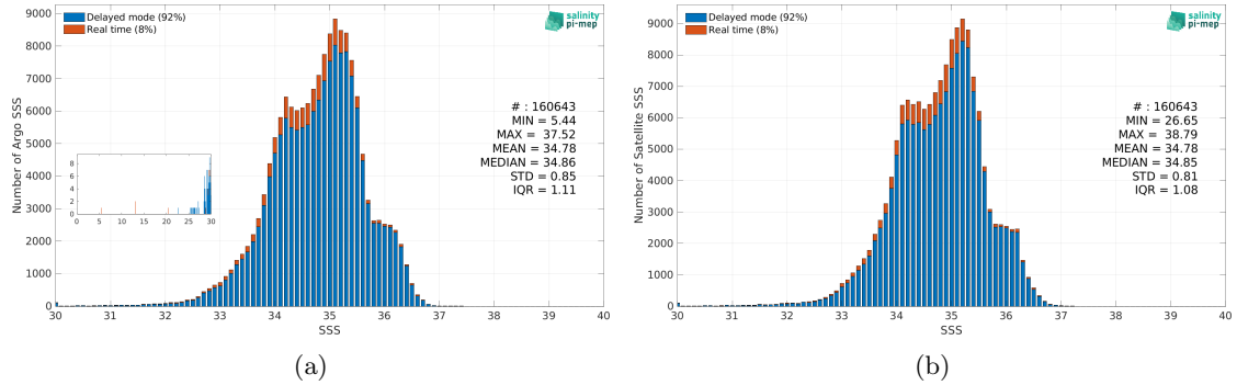
Figure 2: Histograms of SSS from Argo (a) and CCI SSS L4 Merged-OI v3.2 - 30-day running (ESA) (b) considering all match-up pairs per bins of 0.1 over the Equatorial Ocean 10N-10S Pi-MEP region and for the full satellite product period.
