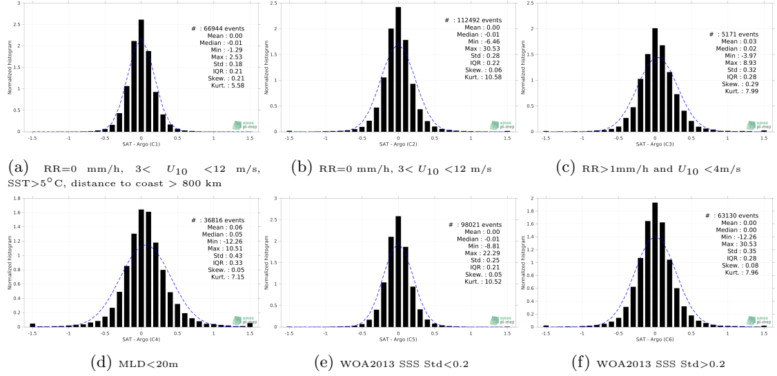
Figure 13: Normalized histogram of \Delta SSS (CCI SSS L4 Merged-OI v3.2 - 30-day running (ESA) - Argo) for 6 different subdatasets corresponding to: RR=0 mm/h, 3 < U_{10} < 12 m/s, SST>5°C, distance to coast > 800 km (a), RR=0 mm/h, 3 < U_{10} < 12 m/s (b), RR>1mm/h and U_{10} < 4 m/s (c), MLD<20m (d), WOA2013 SSS Std<0.2 (e), WOA2013 SSS Std>0.2 (f).
