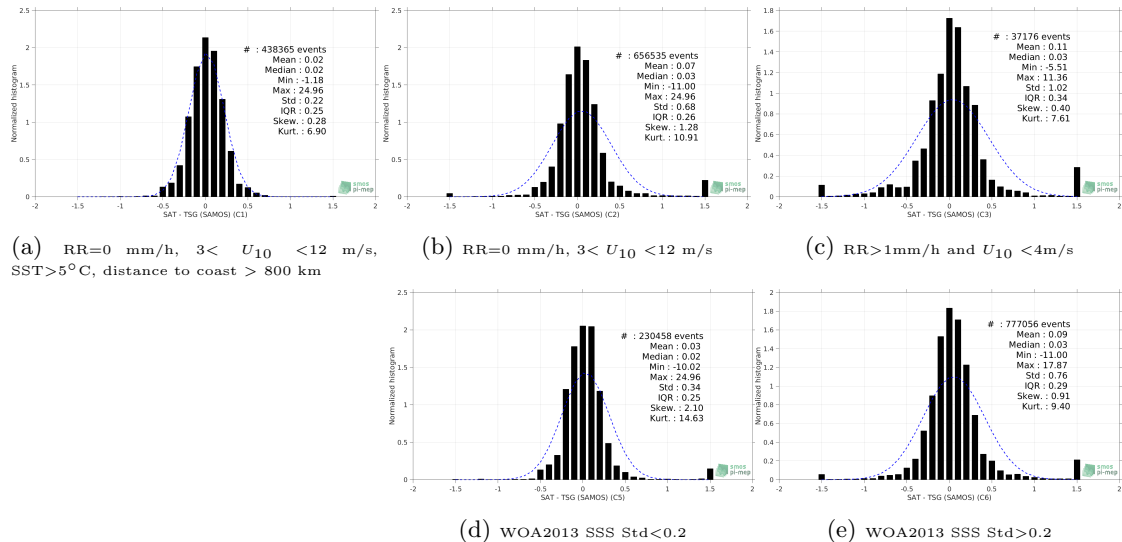
Figure 13: Normalized histogram of \Delta SSS (CCI SSS L4 Merged-OI v2.31 - 7-day running (ESA) - TSG (SAMOS)) for 5 different subdatasets corresponding to: RR=0 mm/h, 3 < U_{10} < 12 m/s, SST >5^\circ\text{C} , distance to coast > 800 km (a), RR=0 mm/h, 3 < U_{10} < 12 m/s (b), RR >1 mm/h and U_{10} < 4 m/s (c), WOA2013 SSS Std <0.2 (d), WOA2013 SSS Std >0.2 (e).
