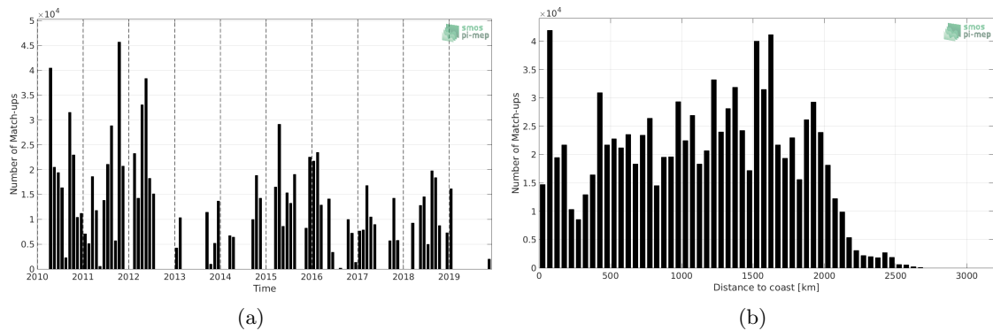
Figure 1: Number of match-ups between TSG (SAMOS) and CCI SSS L4 Merged-OI v2.31 - 7-day running (ESA) SSS as a function of time (a) and as function of the distance to coast (b) over the Equatorial Ocean 10N-10S Pi-MEP region and for the full satellite product period.
