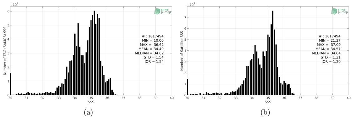
Figure 2: Histograms of SSS from TSG (SAMOS) (a) and CCI SSS L4 Merged-OI v2.31 - 7-day running (ESA) (b) considering all match-up pairs per bins of 0.1 over the Equatorial Ocean 10N-10S Pi-MEP region and for the full satellite product period.
