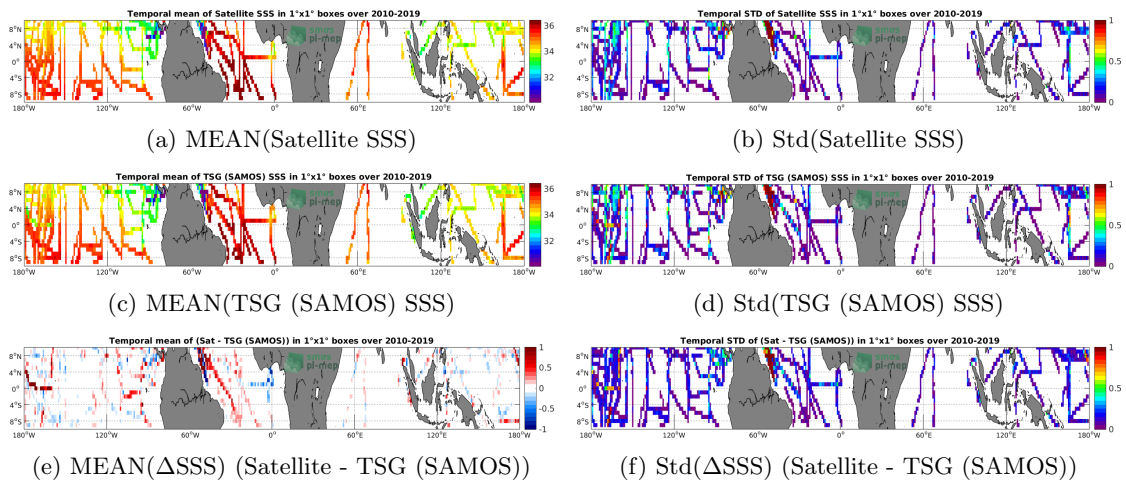
Figure 6: Temporal mean (left) and Std (right) of SSS from CCI SSS L4 Merged-OI v2.31 - 7-day running (ESA) (top), TSG (SAMOS) (middle), and of \Delta SSS (Satellite - TSG (SAMOS)). Only match-up pairs are used to generate these maps.
