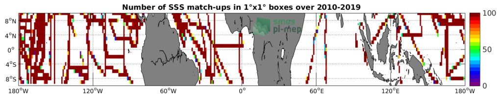
Figure 4: Number of SSS match-ups between TSG (SAMOS) SSS and the CCI SSS L4 Merged-OI v2.31 - 7-day running (ESA) SSS product for the Equatorial Ocean 10N-10S Pi-MEP region over 1^\circ \times 1^\circ boxes and for the full satellite product period.
