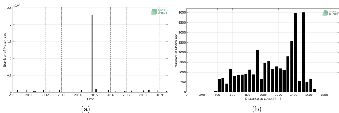
Figure 1: Number of match-ups between TSG (Polarstern) and CCI L4 Merged-OI v2.31 - 7-day running (ESA) SSS as a function of time (a) and as function of the distance to coast (b) over the Equatorial Ocean 10N-10S Pi-MEP region and for the full satellite product period.
