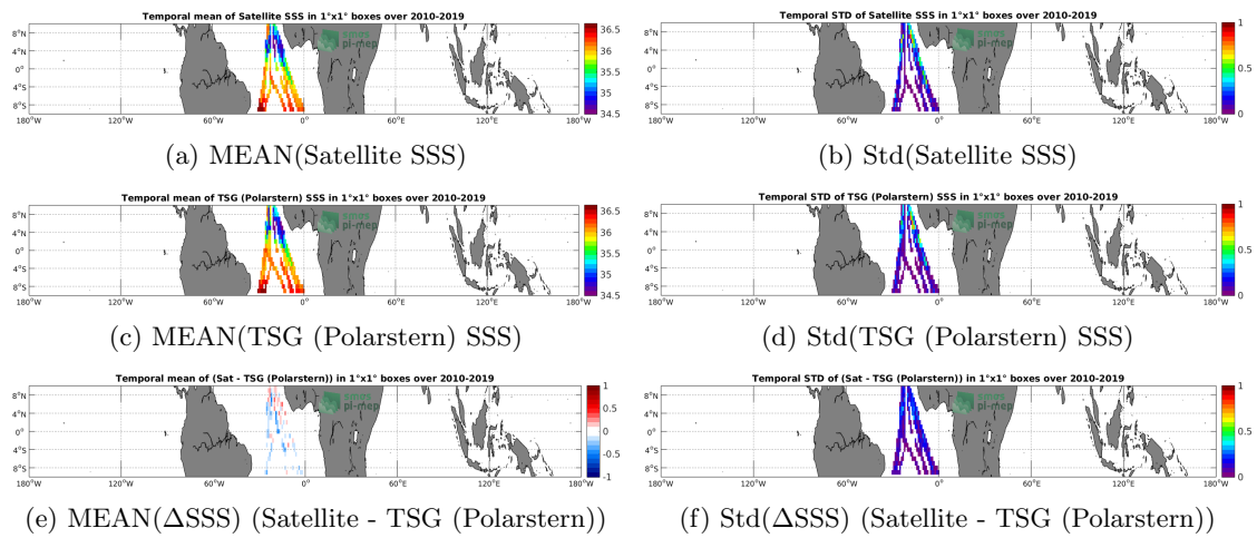
Figure 6: Temporal mean (left) and Std (right) of SSS from CCI L4 Merged-OI v2.31 - 7-day running (ESA) (top), TSG (Polarstern) (middle), and of \Delta SSS (Satellite - TSG (Polarstern)). Only match-up pairs are used to generate these maps.
