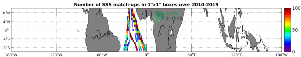
Figure 4: Number of SSS match-ups between TSG (Polarstern) SSS and the CCI L4 Merged-OI v2.31 - 7-day running (ESA) SSS product for the Equatorial Ocean 10N-10S Pi-MEP region over 1°x1° boxes and for the full satellite product period.
