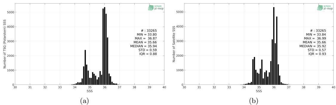
Figure 2: Histograms of SSS from TSG (Polarstern) (a) and CCI L4 Merged-OI v2.31 - 7-day running (ESA) (b) considering all match-up pairs per bins of 0.1 over the Equatorial Ocean 10N-10S Pi-MEP region and for the full satellite product period.
