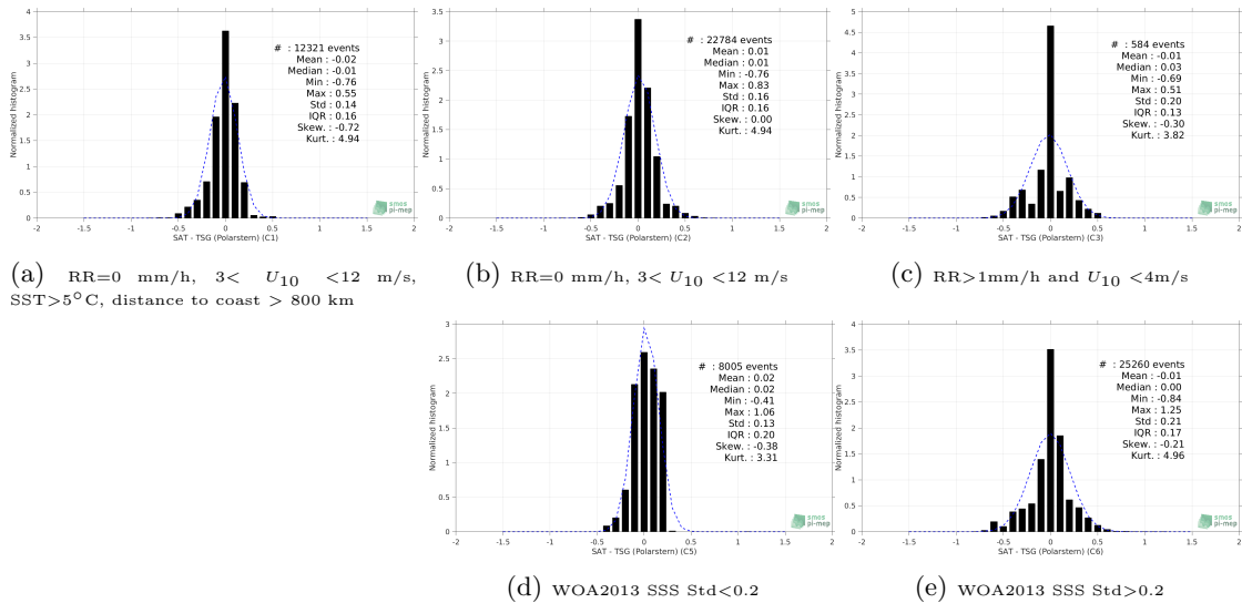
Figure 13: Normalized histogram of \Delta SSS (CCI L4 Merged-OI v2.31 - 7-day running (ESA) - TSG (Polarstern)) for 5 different subdatasets corresponding to: RR=0 mm/h, 3 < U_{10} < 12 m/s, SST >5^\circ\text{C} , distance to coast > 800 km (a), RR=0 mm/h, 3 < U_{10} < 12 m/s (b), RR >1 mm/h and U_{10} < 4 m/s (c), WOA2013 SSS Std <0.2 (d), WOA2013 SSS Std >0.2 (e).
