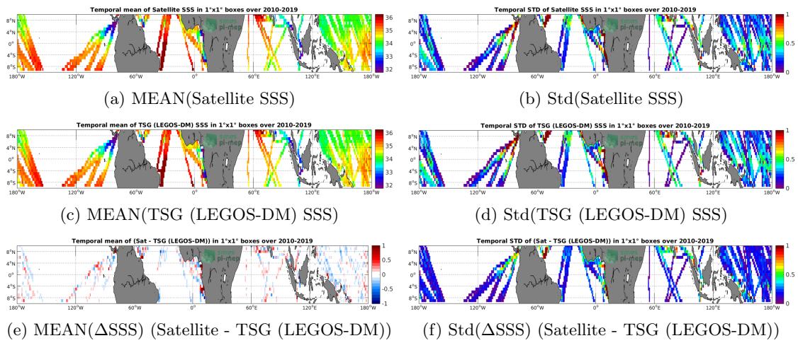
Figure 6: Temporal mean (left) and Std (right) of SSS from CCI SSS L4 Merged-OI v2.31 - 7-day running (ESA) (top), TSG (LEGOS-DM) (middle), and of \Delta SSS (Satellite - TSG (LEGOS-DM)). Only match-up pairs are used to generate these maps.
