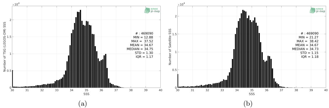
Figure 2: Histograms of SSS from TSG (LEGOS-DM) (a) and CCI SSS L4 Merged-OI v2.31 - 7-day running (ESA) (b) considering all match-up pairs per bins of 0.1 over the Equatorial Ocean 10N-10S Pi-MEP region and for the full satellite product period.
