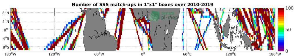
Figure 4: Number of SSS match-ups between TSG (LEGOS-DM) SSS and the CCI SSS L4 Merged-OI v2.31 - 7-day running (ESA) SSS product for the Equatorial Ocean 10N-10S Pi-MEP region over 1^\circ \times 1^\circ boxes and for the full satellite product period.
