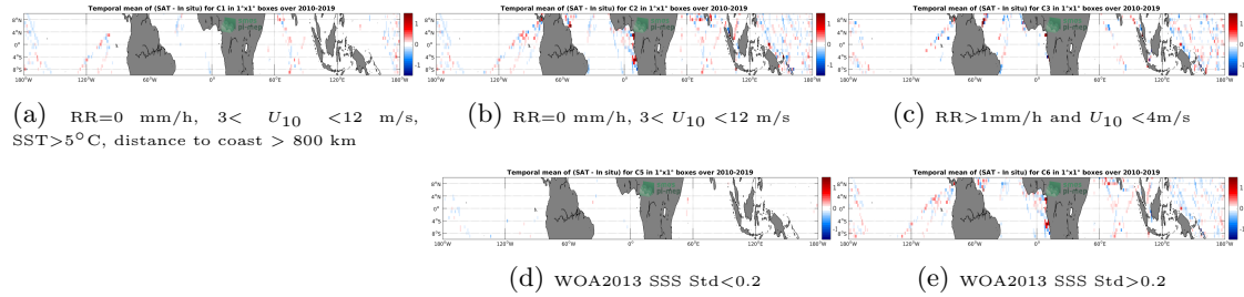
Figure 12: Temporal mean gridded over spatial boxes of size 1^{\circ}\times 1^{\circ} of \Delta\text{SSS} (CCI SSS L4 Merged-OI v2.31 - 7-day running (ESA) - TSG (LEGOS-DM)) for 5 different subdatasets corresponding to:RR=0 mm/h, 3 < U_{10} < 12 m/s, SST >5^{\circ}\text{C} , distance to coast > 800 km (a), RR=0 mm/h, 3 < U_{10} < 12 m/s (b), RR >1 mm/h and U_{10} < 4 m/s (c), WOA2013 SSS Std <0.2 (d), WOA2013 SSS Std >0.2 (e).
