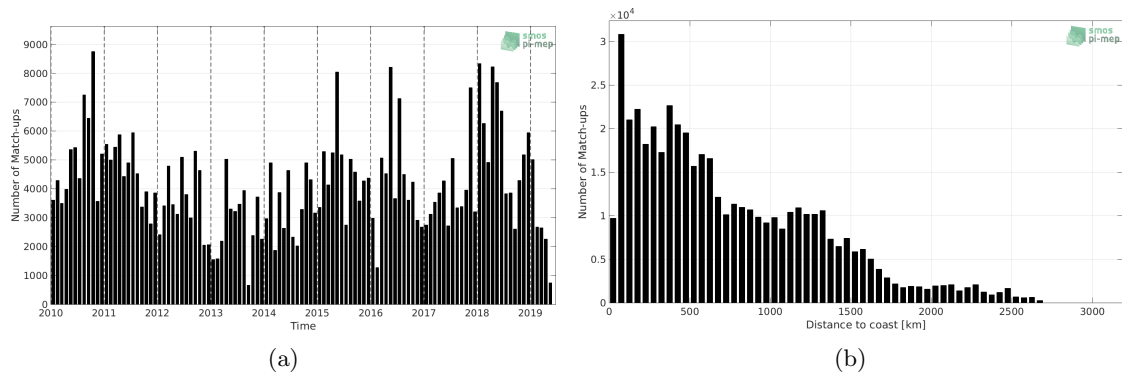
Figure 1: Number of match-ups between TSG (LEGOS-DM) and CCI SSS L4 Merged-OI v2.31 - 7-day running (ESA) SSS as a function of time (a) and as function of the distance to coast (b) over the Equatorial Ocean 10N-10S Pi-MEP region and for the full satellite product period.
