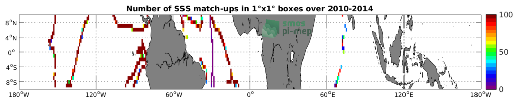
Figure 4: Number of SSS match-ups between TSG (GOSUD-Sailing-ship) SSS and the CCI SSS L4 Merged-OI v2.31 - 7-day running (ESA) SSS product for the Equatorial Ocean 10N-10S Pi-MEP region over 1°x1° boxes and for the full satellite product period.
