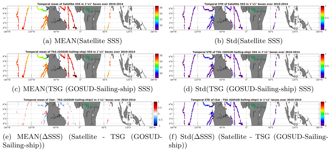
Figure 6: Temporal mean (left) and Std (right) of SSS from CCI SSS L4 Merged-OI v2.31 - 7-day running (ESA) (top), TSG (GOSUD-Sailing-ship) (middle), and of \Delta SSS (Satellite - TSG (GOSUD-Sailing-ship)). Only match-up pairs are used to generate these maps.
