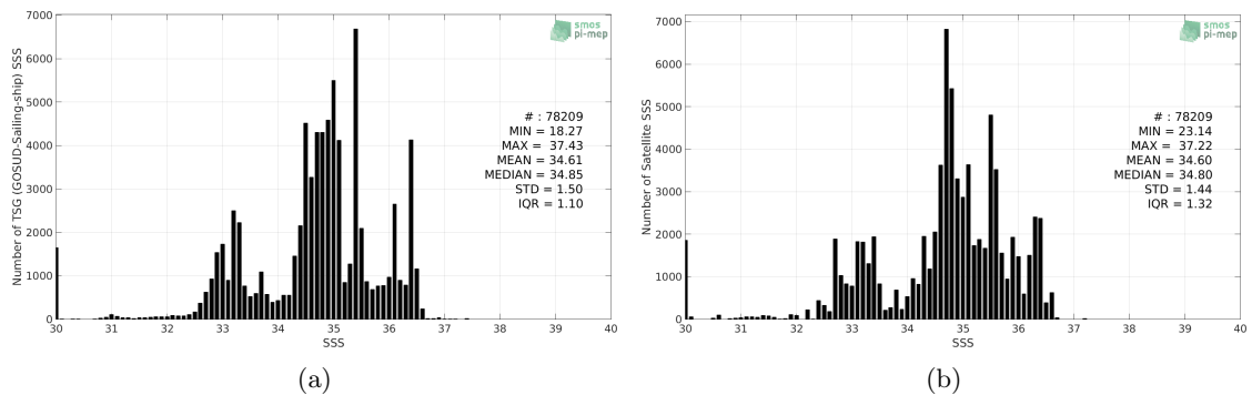
Figure 2: Histograms of SSS from TSG (GOSUD-Sailing-ship) (a) and CCI SSS L4 Merged-OI v2.31 - 7-day running (ESA) (b) considering all match-up pairs per bins of 0.1 over the Equatorial Ocean 10N-10S Pi-MEP region and for the full satellite product period.
