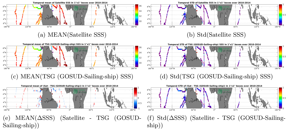
Figure 6: Temporal mean (left) and Std (right) of SSS from CCI L4 Merged-OI v2.31 - 7-day running (ESA) (top), TSG (GOSUD-Sailing-ship) (middle), and of \Delta SSS (Satellite - TSG (GOSUD-Sailing-ship)). Only match-up pairs are used to generate these maps.
