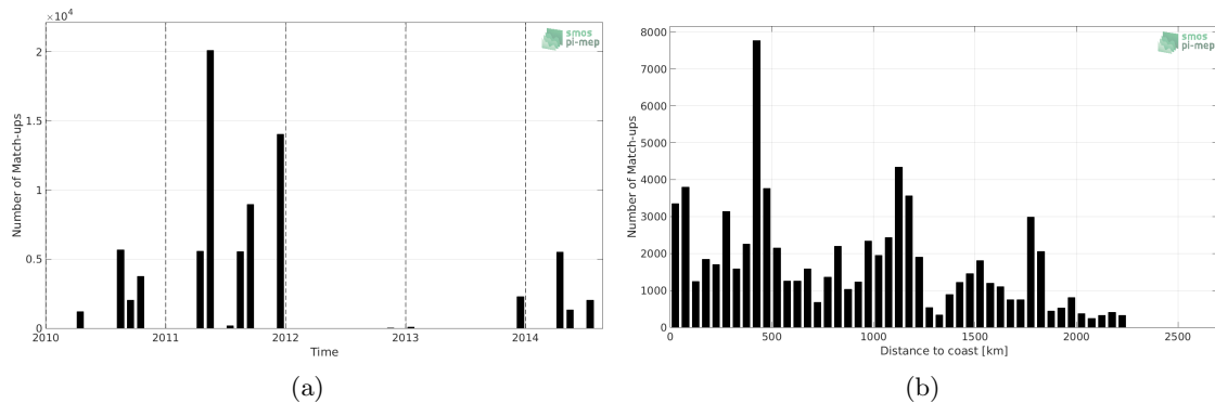
Figure 1: Number of match-ups between TSG (GOSUD-Sailing-ship) and CCI L4 Merged-OI v2.31 - 7-day running (ESA) SSS as a function of time (a) and as function of the distance to coast (b) over the Equatorial Ocean 10N-10S Pi-MEP region and for the full satellite product period.
