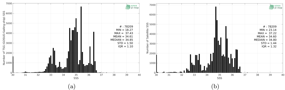
Figure 2: Histograms of SSS from TSG (GOSUD-Sailing-ship) (a) and CCI L4 Merged-OI v2.31 - 7-day running (ESA) (b) considering all match-up pairs per bins of 0.1 over the Equatorial Ocean 10N-10S Pi-MEP region and for the full satellite product period.
