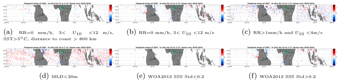
Figure 12: Temporal mean gridded over spatial boxes of size 1^\circ \times 1^\circ of \Delta SSS (CCI SSS L4 Merged-OI v2.31 - 7-day running (ESA) - Argo) for 6 different subdatasets corresponding to:RR=0 mm/h, 3 < U_{10} < 12 m/s, SST >5^\circ C, distance to coast > 800 km (a), RR=0 mm/h, 3 < U_{10} < 12 m/s (b), RR >1 mm/h and U_{10} < 4 m/s (c),MLD <20 m (d),WOA2013 SSS Std <0.2 (e),WOA2013 SSS Std >0.2 (f).
