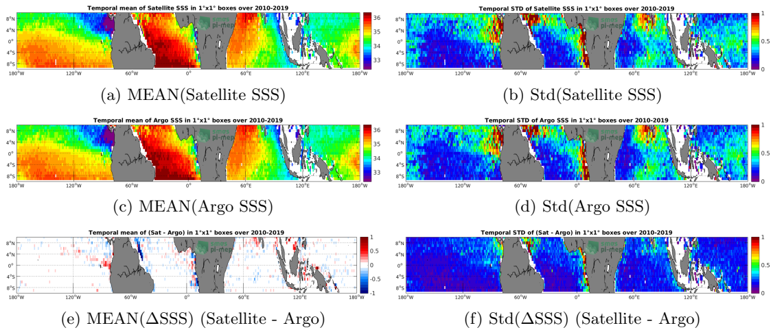
Figure 6: Temporal mean (left) and Std (right) of SSS from CCI SSS L4 Merged-OI v2.31 - 7-day running (ESA) (top), Argo (middle), and of \Delta SSS (Satellite - Argo). Only match-up pairs are used to generate these maps.
