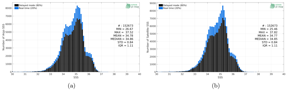
Figure 2: Histograms of SSS from Argo (a) and CCI SSS L4 Merged-OI v2.31 - 7-day running (ESA) (b) considering all match-up pairs per bins of 0.1 over the Equatorial Ocean 10N-10S Pi-MEP region and for the full satellite product period.
