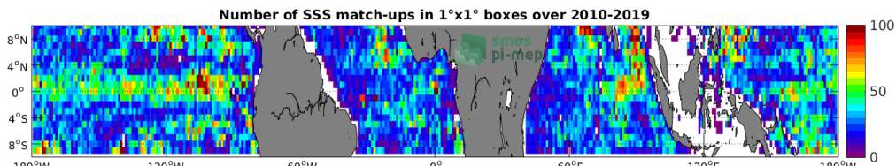
Figure 4: Number of SSS match-ups between Argo SSS and the CCI SSS L4 Merged-OI v2.31 - 7-day running (ESA) SSS product for the Equatorial Ocean 10N-10S Pi-MEP region over 1°x1° boxes and for the full satellite product period.
