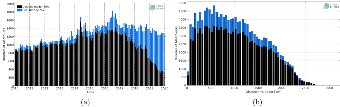
Figure 1: Number of match-ups between Argo and CCI SSS L4 Merged-OI v2.31 - 7-day running (ESA) SSS as a function of time (a) and as function of the distance to coast (b) over the Equatorial Ocean 10N-10S Pi-MEP region and for the full satellite product period.
