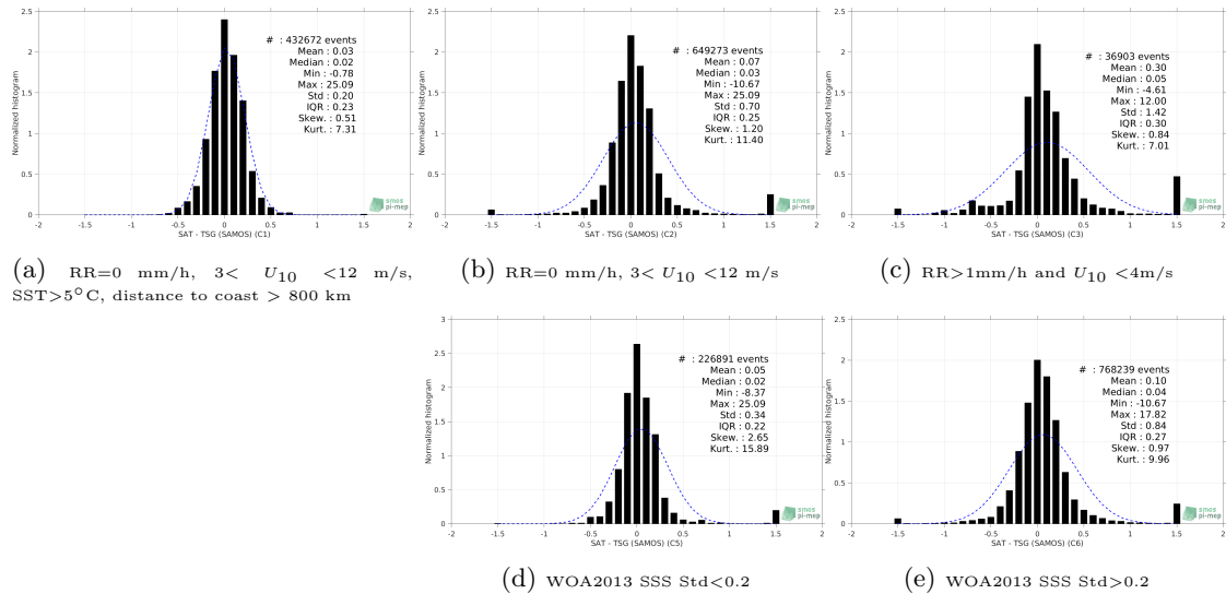
Figure 13: Normalized histogram of \Delta SSS (CCI L4 Merged-OI v2.31 - 30-day running (ESA) - TSG (SAMOS)) for 5 different subdatasets corresponding to: RR=0 mm/h, 3 < U_{10} < 12 m/s, SST >5^\circ\text{C} , distance to coast > 800 km (a), RR=0 mm/h, 3 < U_{10} < 12 m/s (b), RR >1 mm/h and U_{10} < 4 m/s (c), WOA2013 SSS Std <0.2 (d), WOA2013 SSS Std >0.2 (e).
