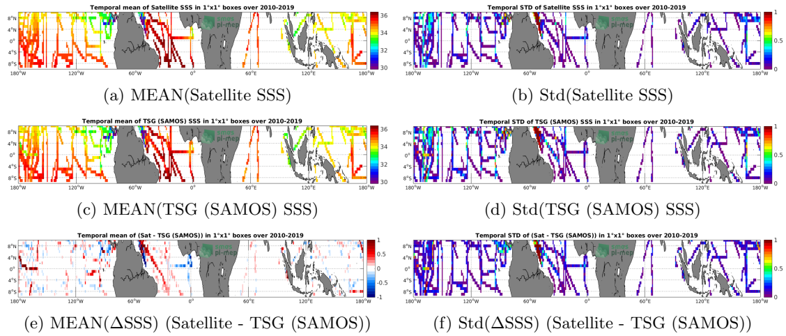
Figure 6: Temporal mean (left) and Std (right) of SSS from CCI L4 Merged-OI v2.31 - 30-day running (ESA) (top), TSG (SAMOS) (middle), and of \Delta SSS (Satellite - TSG (SAMOS)). Only match-up pairs are used to generate these maps.
