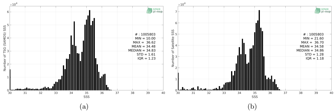
Figure 2: Histograms of SSS from TSG (SAMOS) (a) and CCI L4 Merged-OI v2.31 - 30-day running (ESA) (b) considering all match-up pairs per bins of 0.1 over the Equatorial Ocean 10N-10S Pi-MEP region and for the full satellite product period.
