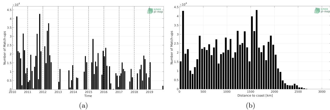
Figure 1: Number of match-ups between TSG (SAMOS) and CCI L4 Merged-OI v2.31 - 30-day running (ESA) SSS as a function of time (a) and as function of the distance to coast (b) over the Equatorial Ocean 10N-10S Pi-MEP region and for the full satellite product period.
