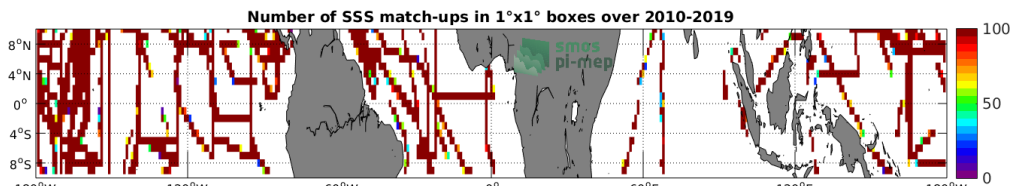
Figure 4: Number of SSS match-ups between TSG (SAMOS) SSS and the CCI L4 Merged-OI v2.31 - 30-day running (ESA) SSS product for the Equatorial Ocean 10N-10S Pi-MEP region over 1°x1° boxes and for the full satellite product period.
