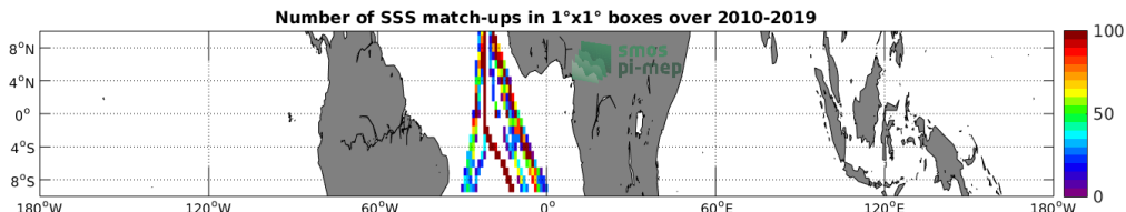
Figure 4: Number of SSS match-ups between TSG (Polarstern) SSS and the CCI SSS L4 Merged-OI v2.31 - 30-day running (ESA) SSS product for the Equatorial Ocean 10N-10S Pi-MEP region over 1°x1° boxes and for the full satellite product period.
