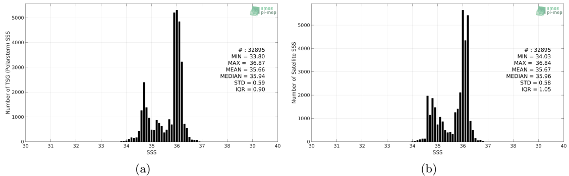
Figure 2: Histograms of SSS from TSG (Polarstern) (a) and CCI SSS L4 Merged-OI v2.31 - 30-day running (ESA) (b) considering all match-up pairs per bins of 0.1 over the Equatorial Ocean 10N-10S Pi-MEP region and for the full satellite product period.
