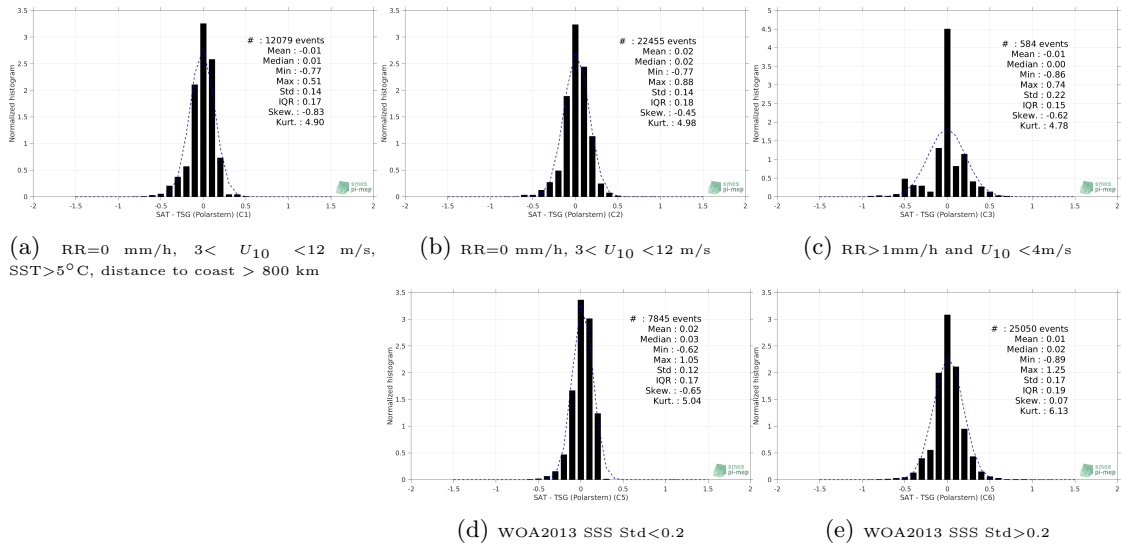
Figure 13: Normalized histogram of ΔSSS (CCI SSS L4 Merged-OI v2.31 - 30-day running (ESA) - TSG (Polarstern)) for 5 different subdatasets corresponding to: RR=0 mm/h, 3 < U 10 < 12 m/s, SST>5°C, distance to coast > 800 km (a), RR=0 mm/h, 3 < U 10 < 12 m/s (b), RR>1mm/h and U 10 < 4m/s (c), WOA2013 SSS Std<0.2 (d), WOA2013 SSS Std>0.2 (e).
