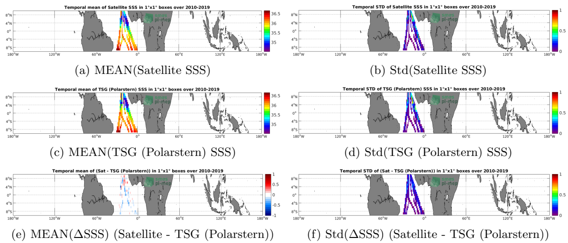
Figure 6: Temporal mean (left) and Std (right) of SSS from CCI SSS L4 Merged-OI v2.31 - 30-day running (ESA) (top), TSG (Polarstern) (middle), and of \Delta SSS (Satellite - TSG (Polarstern)). Only match-up pairs are used to generate these maps.
