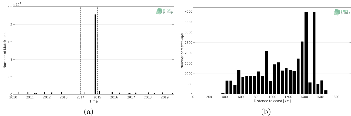
Figure 1: Number of match-ups between TSG (Polarstern) and CCI L4 Merged-OI v2.31 - 30-day running (ESA) SSS as a function of time (a) and as function of the distance to coast (b) over the Equatorial Ocean 10N-10S Pi-MEP region and for the full satellite product period.
