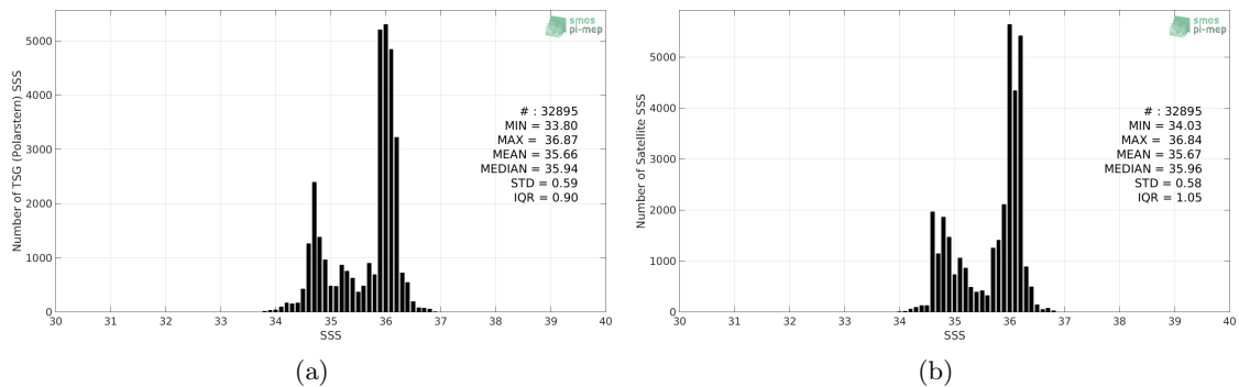
Figure 2: Histograms of SSS from TSG (Polarstern) (a) and CCI L4 Merged-OI v2.31 - 30-day running (ESA) (b) considering all match-up pairs per bins of 0.1 over the Equatorial Ocean 10N-10S Pi-MEP region and for the full satellite product period.
