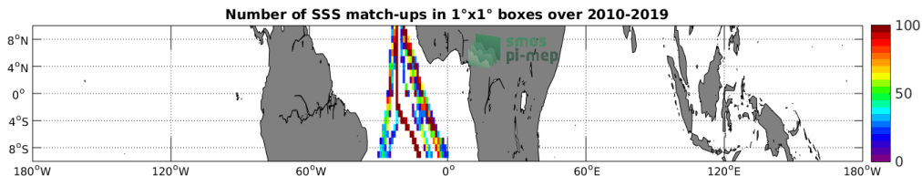
Figure 4: Number of SSS match-ups between TSG (Polarstern) SSS and the CCI L4 Merged-OI v2.31 - 30-day running (ESA) SSS product for the Equatorial Ocean 10N-10S Pi-MEP region over 1°x1° boxes and for the full satellite product period.
