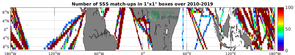
Figure 4: Number of SSS match-ups between TSG (LEGOS-DM) SSS and the CCI SSS L4 Merged-OI v2.31 - 30-day running (ESA) SSS product for the Equatorial Ocean 10N-10S Pi-MEP region over 1°x1° boxes and for the full satellite product period.
