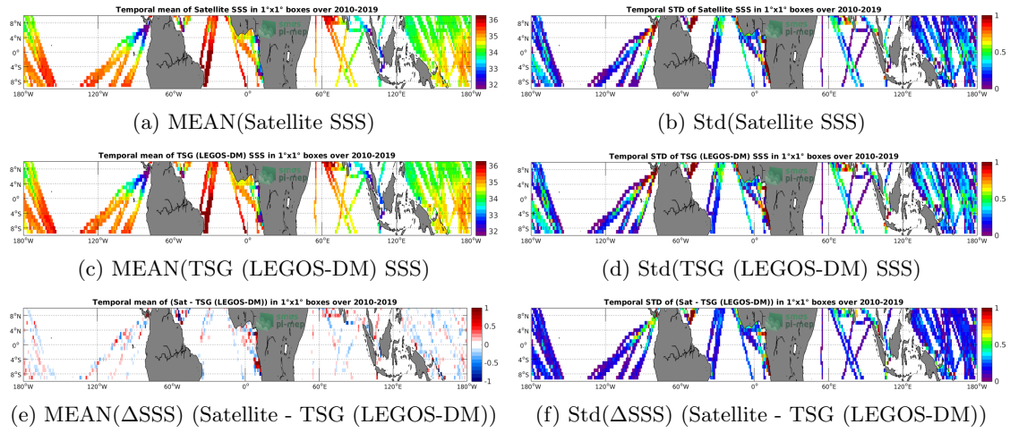
Figure 6: Temporal mean (left) and Std (right) of SSS from CCI SSS L4 Merged-OI v2.31 - 30-day running (ESA) (top), TSG (LEGOS-DM) (middle), and of \Delta SSS (Satellite - TSG (LEGOS-DM)). Only match-up pairs are used to generate these maps.
