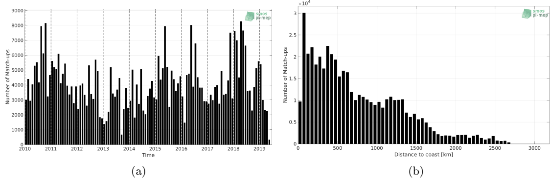
Figure 1: Number of match-ups between TSG (LEGOS-DM) and CCI SSS L4 Merged-OI v2.31 - 30-day running (ESA) SSS as a function of time (a) and as function of the distance to coast (b) over the Equatorial Ocean 10N-10S Pi-MEP region and for the full satellite product period.
