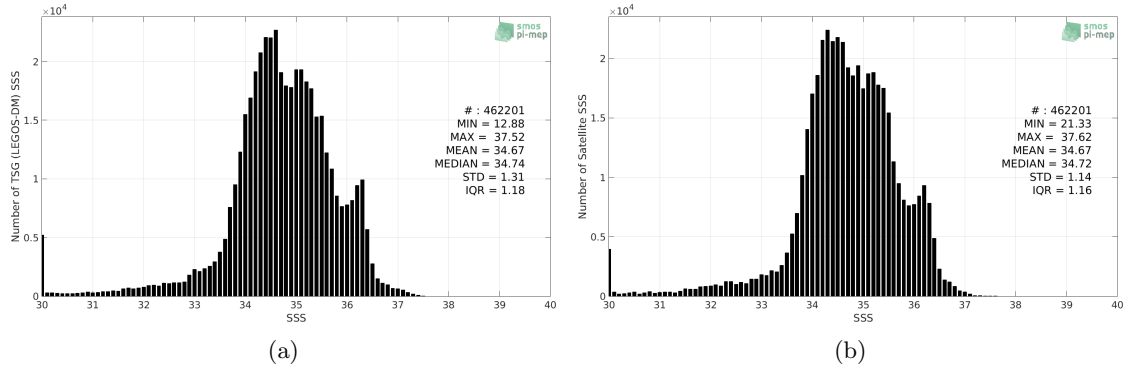
Figure 2: Histograms of SSS from TSG (LEGOS-DM) (a) and CCI SSS L4 Merged-OI v2.31 - 30-day running (ESA) (b) considering all match-up pairs per bins of 0.1 over the Equatorial Ocean 10N-10S Pi-MEP region and for the full satellite product period.
