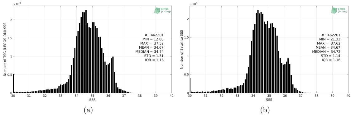
Figure 2: Histograms of SSS from TSG (LEGOS-DM) (a) and CCI L4 Merged-OI v2.31 - 30-day running (ESA) (b) considering all match-up pairs per bins of 0.1 over the Equatorial Ocean 10N-10S Pi-MEP region and for the full satellite product period.
