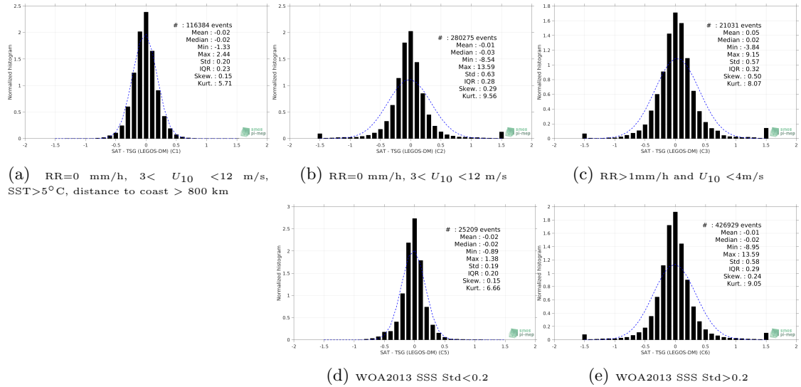
Figure 13: Normalized histogram of \Delta SSS (CCI L4 Merged-OI v2.31 - 30-day running (ESA) - TSG (LEGOS-DM)) for 5 different subdatasets corresponding to: RR=0 mm/h, 3 < U_{10} < 12 m/s, SST >5^\circ\text{C} , distance to coast > 800 km (a), RR=0 mm/h, 3 < U_{10} < 12 m/s (b), RR >1 mm/h and U_{10} < 4 m/s (c), WOA2013 SSS Std <0.2 (d), WOA2013 SSS Std >0.2 (e).
