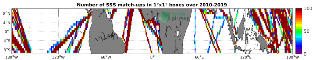
Figure 4: Number of SSS match-ups between TSG (LEGOS-DM) SSS and the CCI L4 Merged-OI v2.31 - 30-day running (ESA) SSS product for the Equatorial Ocean 10N-10S Pi-MEP region over 1°x1° boxes and for the full satellite product period.
