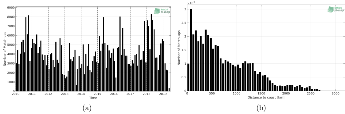
Figure 1: Number of match-ups between TSG (LEGOS-DM) and CCI L4 Merged-OI v2.31 - 30-day running (ESA) SSS as a function of time (a) and as function of the distance to coast (b) over the Equatorial Ocean 10N-10S Pi-MEP region and for the full satellite product period.
