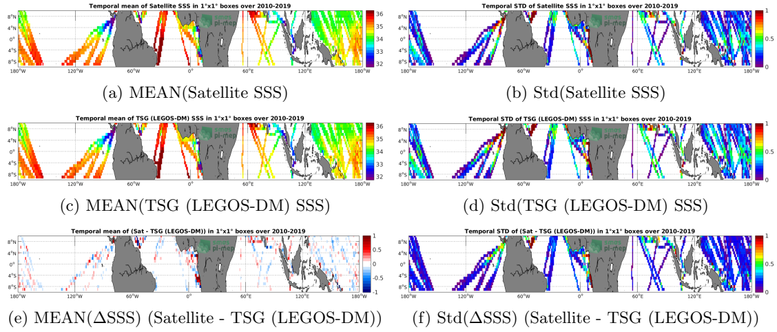
Figure 6: Temporal mean (left) and Std (right) of SSS from CCI L4 Merged-OI v2.31 - 30-day running (ESA) (top), TSG (LEGOS-DM) (middle), and of \Delta SSS (Satellite - TSG (LEGOS-DM)). Only match-up pairs are used to generate these maps.
