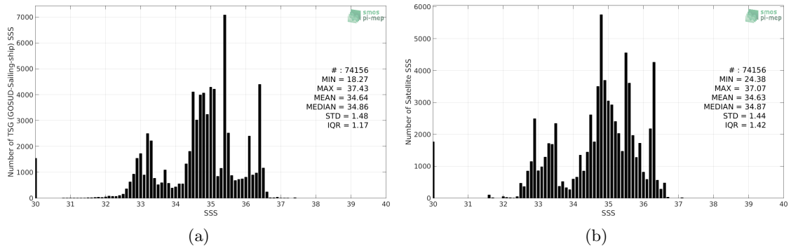
Figure 2: Histograms of SSS from TSG (GOSUD-Sailing-ship) (a) and CCI SSS L4 Merged-OI v2.31 - 30-day running (ESA) (b) considering all match-up pairs per bins of 0.1 over the Equatorial Ocean 10N-10S Pi-MEP region and for the full satellite product period.
