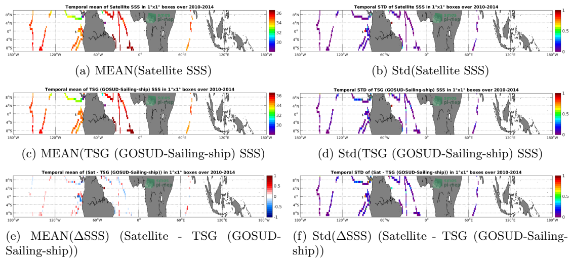
Figure 6: Temporal mean (left) and Std (right) of SSS from CCI L4 Merged-OI v2.31 - 30-day running (ESA) (top), TSG (GOSUD-Sailing-ship) (middle), and of \Delta SSS (Satellite - TSG (GOSUD-Sailing-ship)). Only match-up pairs are used to generate these maps.
