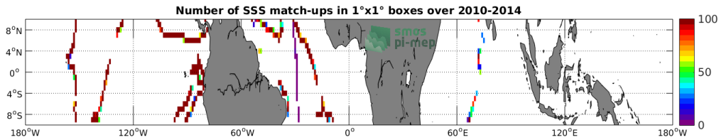
Figure 4: Number of SSS match-ups between TSG (GOSUD-Sailing-ship) SSS and the CCI L4 Merged-OI v2.31 - 30-day running (ESA) SSS product for the Equatorial Ocean 10N-10S Pi-MEP region over 1°x1° boxes and for the full satellite product period.
