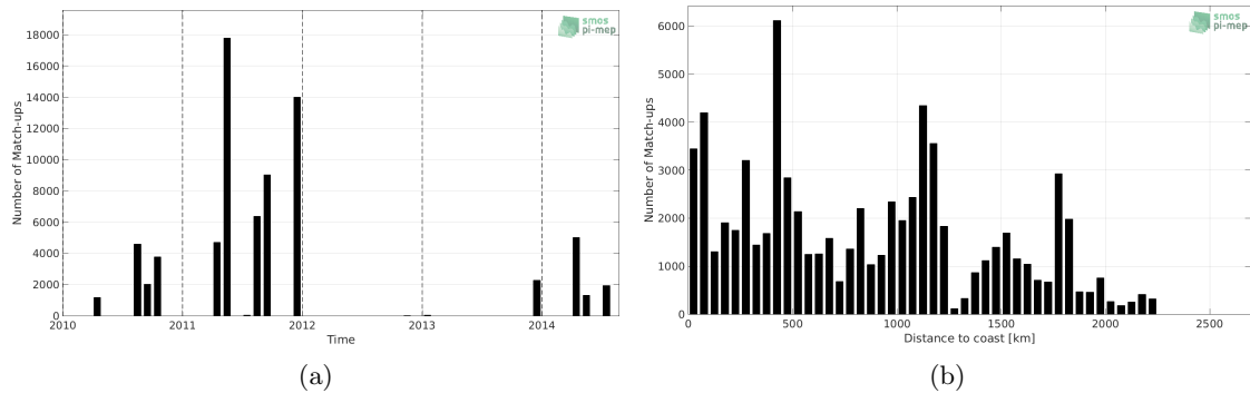
Figure 1: Number of match-ups between TSG (GOSUD-Sailing-ship) and CCI L4 Merged-OI v2.31 - 30-day running (ESA) SSS as a function of time (a) and as function of the distance to coast (b) over the Equatorial Ocean 10N-10S Pi-MEP region and for the full satellite product period.
