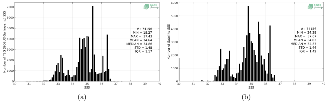
Figure 2: Histograms of SSS from TSG (GOSUD-Sailing-ship) (a) and CCI L4 Merged-OI v2.31 - 30-day running (ESA) (b) considering all match-up pairs per bins of 0.1 over the Equatorial Ocean 10N-10S Pi-MEP region and for the full satellite product period.
