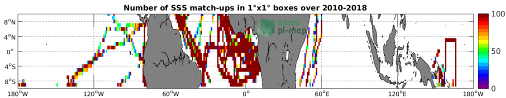
Figure 4: Number of SSS match-ups between TSG (GOSUD-Research-vessel) SSS and the CCI SSS L4 Merged-OI v2.31 - 30-day running (ESA) SSS product for the Equatorial Ocean 10N-10S Pi-MEP region over 1^\circ \times 1^\circ boxes and for the full satellite product period.
