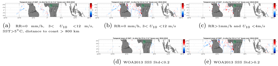
Figure 12: Temporal mean gridded over spatial boxes of size 1^\circ \times 1^\circ of \Delta SSS (CCI SSS L4 Merged-OI v2.31 - 30-day running (ESA) - TSG (GOSUD-Research-vessel)) for 5 different subdatasets corresponding to:RR=0 mm/h, 3 < U_{10} < 12 m/s, SST >5^\circ\text{C} , distance to coast > 800 km (a), RR=0 mm/h, 3 < U_{10} < 12 m/s (b), RR >1 mm/h and U_{10} < 4 m/s (c), WOA2013 SSS Std <0.2 (d), WOA2013 SSS Std >0.2 (e).
