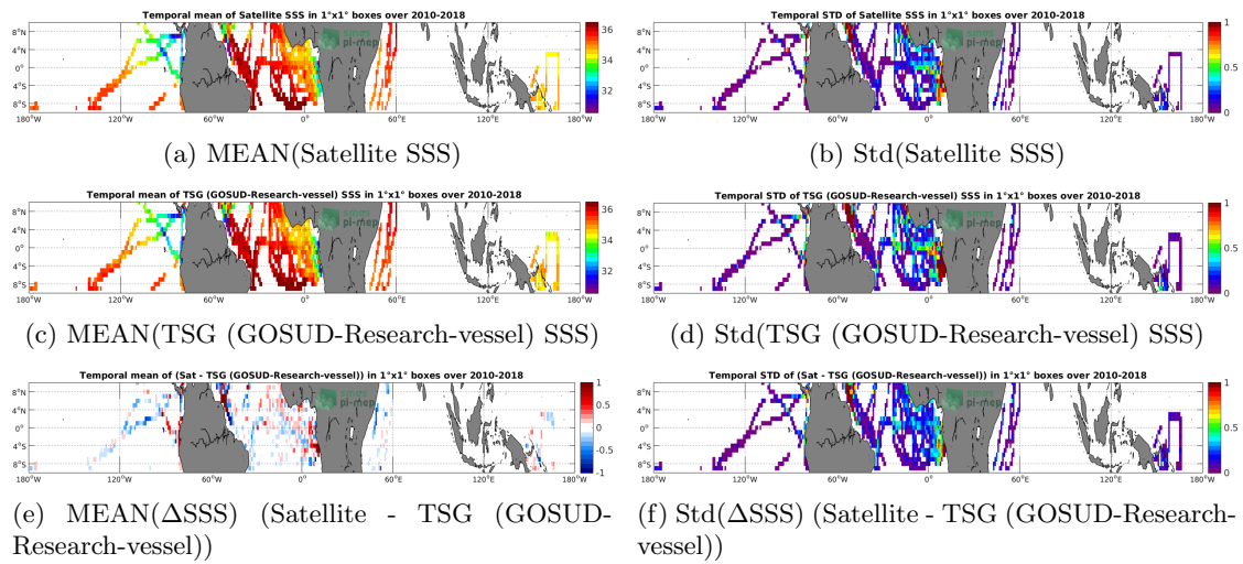
Figure 6: Temporal mean (left) and Std (right) of SSS from CCI SSS L4 Merged-OI v2.31 - 30-day running (ESA) (top), TSG (GOSUD-Research-vessel) (middle), and of \Delta SSS (Satellite - TSG (GOSUD-Research-vessel)). Only match-up pairs are used to generate these maps.
