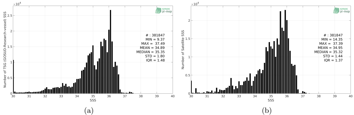
Figure 2: Histograms of SSS from TSG (GOSUD-Research-vessel) (a) and CCI SSS L4 Merged-OI v2.31 - 30-day running (ESA) (b) considering all match-up pairs per bins of 0.1 over the Equatorial Ocean 10N-10S Pi-MEP region and for the full satellite product period.
