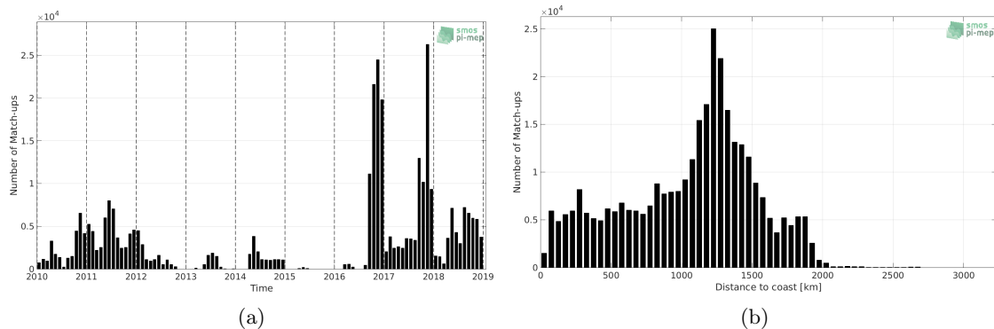
Figure 1: Number of match-ups between Surface drifters and CCI SSS L4 Merged-OI v2.31 - 30-day running (ESA) SSS as a function of time (a) and as function of the distance to coast (b) over the Equatorial Ocean 10N-10S Pi-MEP region and for the full satellite product period.
