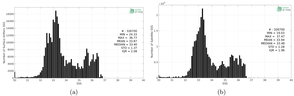
Figure 2: Histograms of SSS from Surface drifters (a) and CCI SSS L4 Merged-OI v2.31 - 30-day running (ESA) (b) considering all match-up pairs per bins of 0.1 over the Equatorial Ocean 10N-10S Pi-MEP region and for the full satellite product period.
