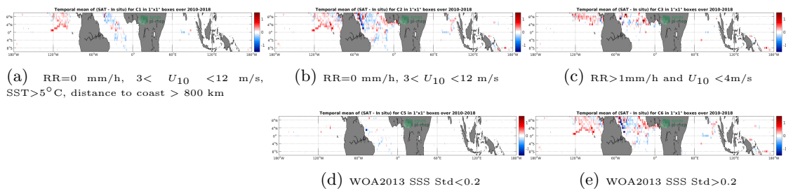
Figure 11: Temporal mean gridded over spatial boxes of size 1^\circ \times 1^\circ of \Delta SSS (CCI SSS L4 Merged-OI v2.31 - 30-day running (ESA) - Surface drifters) for 5 different subdatasets corresponding to: RR=0 mm/h, 3 < U_{10} < 12 m/s, SST >5^\circ\text{C} , distance to coast > 800 km (a), RR=0 mm/h, 3 < U_{10} < 12 m/s (b), RR >1 mm/h and U_{10} < 4 m/s (c), WOA2013 SSS Std <0.2 (d), WOA2013 SSS Std >0.2 (e).
