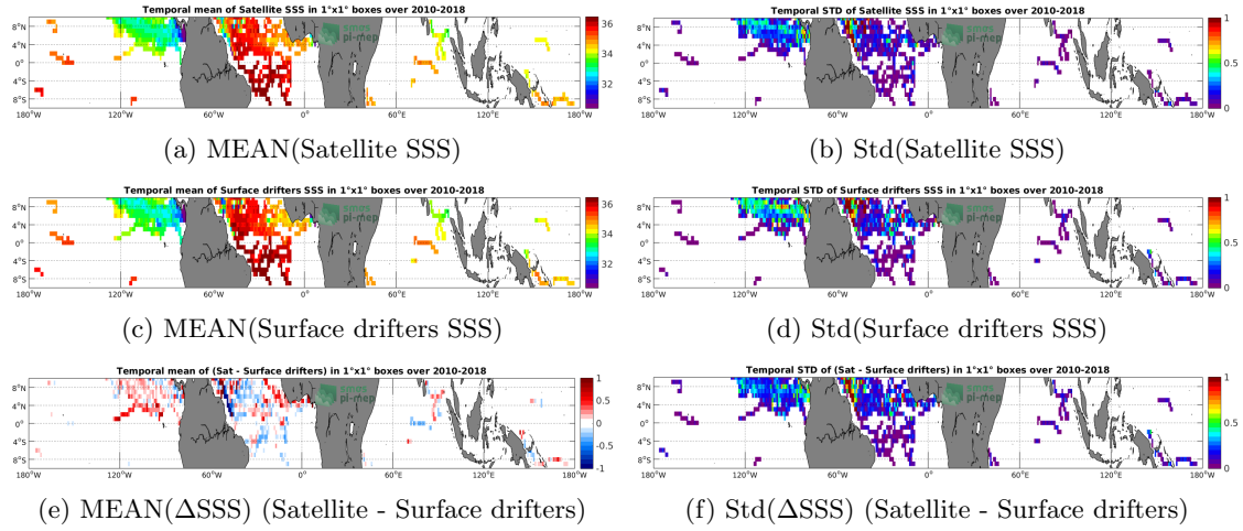
Figure 5: Temporal mean (left) and Std (right) of SSS from CCI SSS L4 Merged-OI v2.31 - 30-day running (ESA) (top), Surface drifters (middle), and of \Delta SSS (Satellite - Surface drifters). Only match-up pairs are used to generate these maps.
