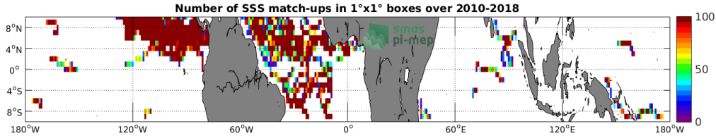
Figure 3: Number of SSS match-ups between Surface drifters SSS and the CCI SSS L4 Merged-OI v2.31 - 30-day running (ESA) SSS product for the Equatorial Ocean 10N-10S Pi-MEP region over 1^\circ \times 1^\circ boxes and for the full satellite product period.
