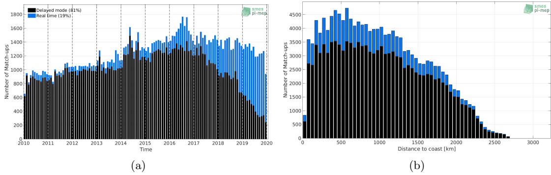
Figure 1: Number of match-ups between Argo and CCI SSS L4 Merged-OI v2.31 - 30-day running (ESA) SSS as a function of time (a) and as function of the distance to coast (b) over the Equatorial Ocean 10N-10S Pi-MEP region and for the full satellite product period.
