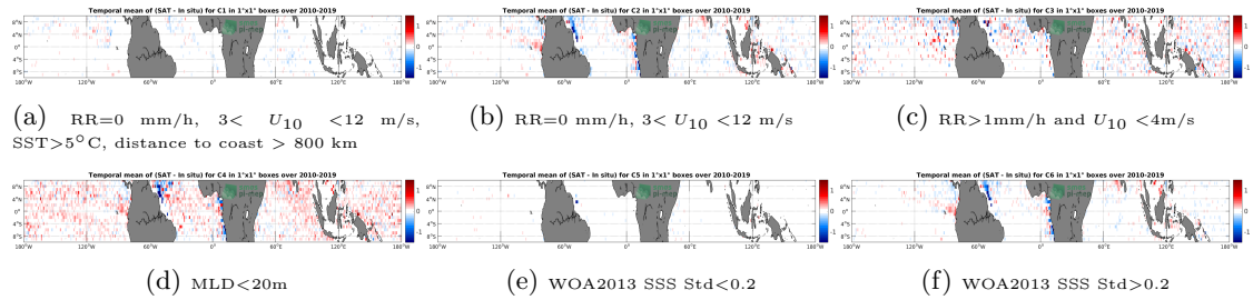
Figure 12: Temporal mean gridded over spatial boxes of size 1^\circ \times 1^\circ of \Delta SSS (CCI SSS L4 Merged-OI v2.31 - 30-day running (ESA) - Argo) for 6 different subdatasets corresponding to:RR=0 mm/h, 3 < U_{10} < 12 m/s, SST >5^\circ C, distance to coast > 800 km (a), RR=0 mm/h, 3 < U_{10} < 12 m/s (b), RR >1 mm/h and U_{10} < 4 m/s (c),MLD <20 m (d),WOA2013 SSS Std <0.2 (e),WOA2013 SSS Std >0.2 (f).
