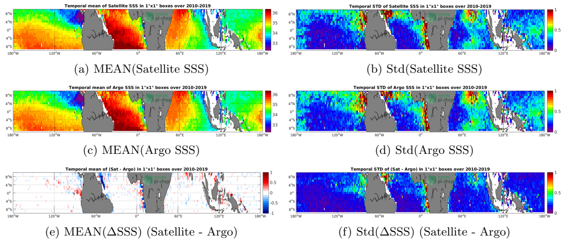
Figure 6: Temporal mean (left) and Std (right) of SSS from CCI SSS L4 Merged-OI v2.31 - 30-day running (ESA) (top), Argo (middle), and of \Delta SSS (Satellite - Argo). Only match-up pairs are used to generate these maps.
