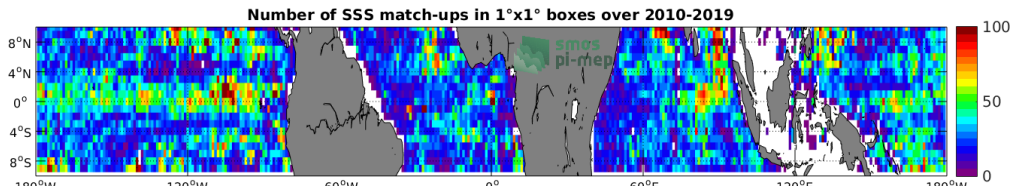
Figure 4: Number of SSS match-ups between Argo SSS and the CCI SSS L4 Merged-OI v2.31 - 30-day running (ESA) SSS product for the Equatorial Ocean 10N-10S Pi-MEP region over 1°x1° boxes and for the full satellite product period.
