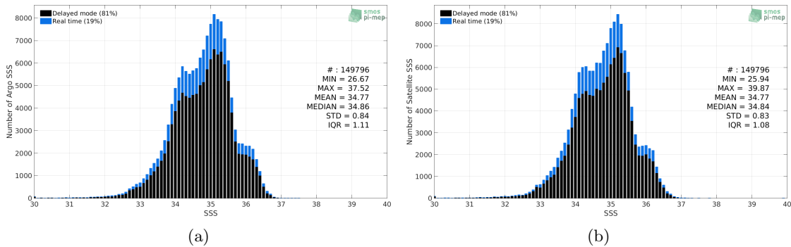
Figure 2: Histograms of SSS from Argo (a) and CCI SSS L4 Merged-OI v2.31 - 30-day running (ESA) (b) considering all match-up pairs per bins of 0.1 over the Equatorial Ocean 10N-10S Pi-MEP region and for the full satellite product period.
