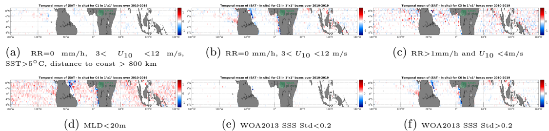
Figure 12: Temporal mean gridded over spatial boxes of size 1^\circ \times 1^\circ of \Delta SSS (CCI L4 Merged-OI v2.31 - 30-day running (ESA) - Argo) for 6 different subdatasets corresponding to:RR=0 mm/h, 3 < U_{10} < 12 m/s, SST >5^\circ\text{C} , distance to coast > 800 km (a), RR=0 mm/h, 3 < U_{10} < 12 m/s (b), RR >1 mm/h and U_{10} < 4 m/s (c),MLD <20 m (d),WOA2013 SSS Std <0.2 (e),WOA2013 SSS Std >0.2 (f).
