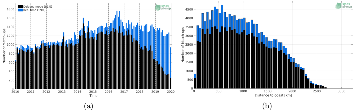
Figure 1: Number of match-ups between Argo and CCI L4 Merged-OI v2.31 - 30-day running (ESA) SSS as a function of time (a) and as function of the distance to coast (b) over the Equatorial Ocean 10N-10S Pi-MEP region and for the full satellite product period.
