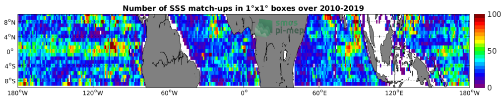
Figure 4: Number of SSS match-ups between Argo SSS and the CCI L4 Merged-OI v2.31 - 30-day running (ESA) SSS product for the Equatorial Ocean 10N-10S Pi-MEP region over 1^\circ \times 1^\circ boxes and for the full satellite product period.
