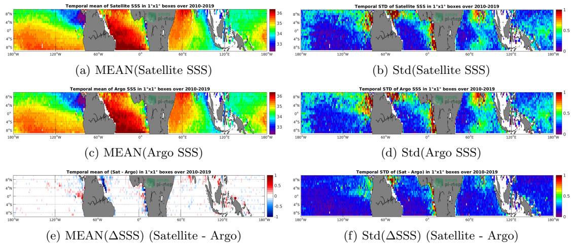
Figure 6: Temporal mean (left) and Std (right) of SSS from CCI L4 Merged-OI v2.31 - 30-day running (ESA) (top), Argo (middle), and of \Delta SSS (Satellite - Argo). Only match-up pairs are used to generate these maps.
