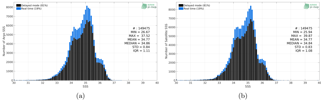
Figure 2: Histograms of SSS from Argo (a) and CCI L4 Merged-OI v2.31 - 30-day running (ESA) (b) considering all match-up pairs per bins of 0.1 over the Equatorial Ocean 10N-10S Pi-MEP region and for the full satellite product period.
