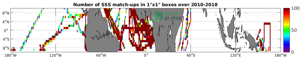
Figure 4: Number of SSS match-ups between TSG-GOSUD-Research-vessel SSS and the CCI-L4-ESA-MERGED-OI-V1.8-30DAY-RUNNING SSS product for the Equatorial Ocean 10N-10S Pi-MEP region over 1°x1° boxes and for the full satellite product period.
