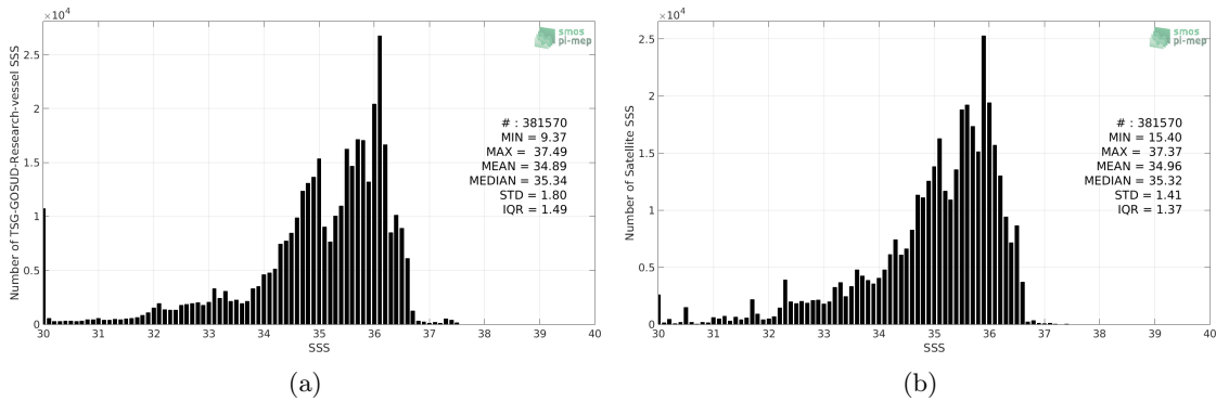
Figure 2: Histograms of SSS from TSG-GOSUD-Research-vessel (a) and CCI-L4-ESA-MERGED-OI-V1.8-30DAY-RUNNING (b) considering all match-up pairs per bins of 0.1 over the Equatorial Ocean 10N-10S Pi-MEP region and for the full satellite product period.
