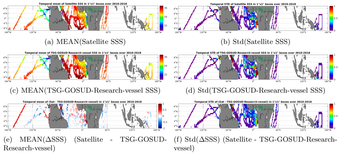
Figure 6: Temporal mean (left) and Std (right) of SSS from CCI-L4-ESA-MERGED-OI-V1.8-30DAY-RUNNING (top), TSG-GOSUD-Research-vessel (middle), and of \Delta SSS (Satellite - TSG-GOSUD-Research-vessel). Only match-up pairs are used to generate these maps.
