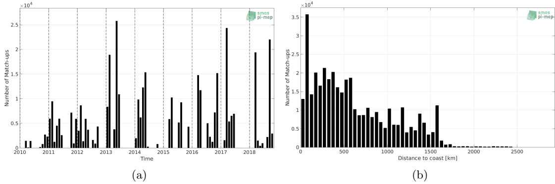
Figure 1: Number of match-ups between TSG-GOSUD-Research-vessel and CCI-L4-ESA-MERGED-OI-V1.8-30DAY-RUNNING SSS as a function of time (a) and as function of the distance to coast (b) over the Equatorial Ocean 10N-10S Pi-MEP region and for the full satellite product period.
