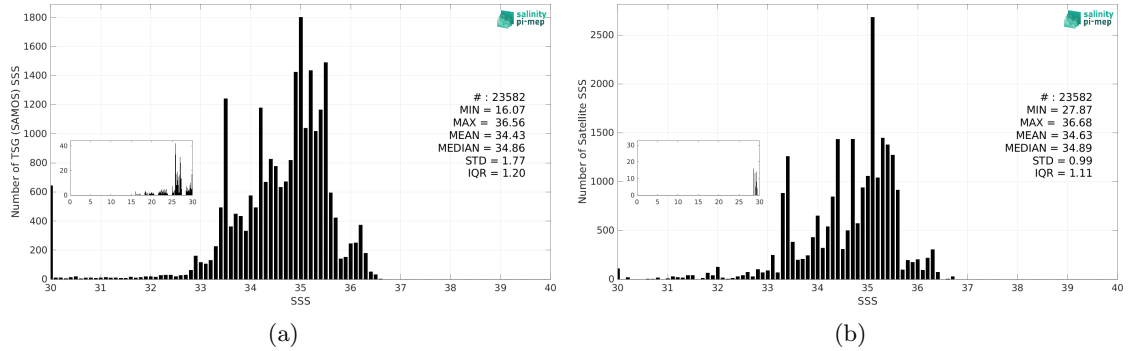
Figure 3: Histograms of SSS from TSG (SAMOS) (a) and Aquarius SSS L4 OI v5 - Weekly (IPRC) (b) considering all match-up pairs per bins of 0.1 over the Equatorial Ocean 10N-10S Pi-MEP region and for the full satellite product period.
