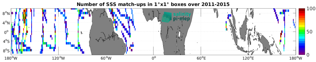
Figure 5: Number of SSS match-ups between TSG (SAMOS) SSS and the Aquarius SSS L4 OI v5 - Weekly (IPRC) SSS product for the Equatorial Ocean 10N-10S Pi-MEP region over 1^\circ \times 1^\circ boxes and for the full satellite product period.
