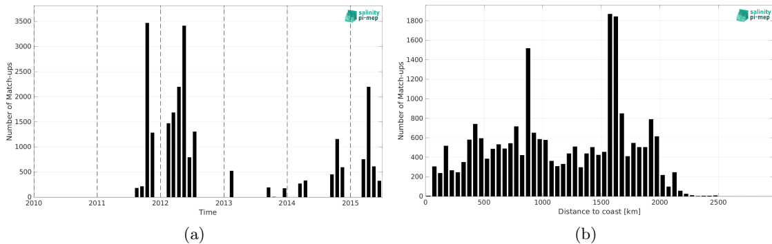
Figure 2: Number of match-ups between TSG (SAMOS) and Aquarius SSS L4 OI v5 - Weekly (IPRC) SSS as a function of time (a) and as function of the distance to coast (b) over the Equatorial Ocean 10N-10S Pi-MEP region and for the full satellite product period.
