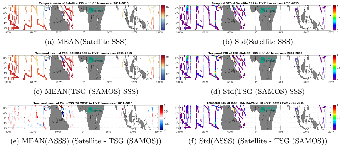
Figure 7: Temporal mean (left) and Std (right) of SSS from Aquarius SSS L4 OI v5 - Weekly (IPRC) (top), TSG (SAMOS) (middle), and of \Delta SSS (Satellite - TSG (SAMOS)). Only match-up pairs are used to generate these maps.
