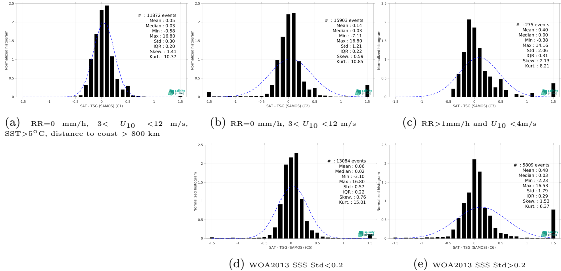
Figure 15: Normalized histogram of \Delta SSS (Aquarius SSS L4 OI v5 - Weekly (IPRC) - TSG (SAMOS)) for 5 different subdatasets corresponding to: RR=0 mm/h, 3 < U_{10} < 12 m/s, SST>5°C, distance to coast > 800 km (a), RR=0 mm/h, 3 < U_{10} < 12 m/s (b), RR>1mm/h and U_{10} < 4 m/s (c), WOA2013 SSS Std<0.2 (d), WOA2013 SSS Std>0.2 (e).
