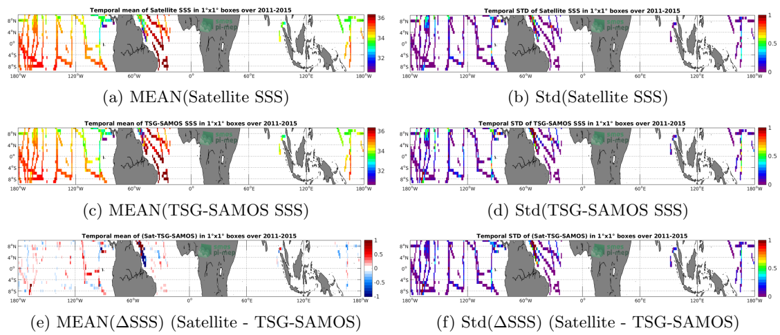
Figure 6: Temporal mean (left) and Std (right) of SSS from Aquarius-L4-IPRC-V5-WEEKLY (top), TSG-SAMOS (middle), and of \Delta SSS (Satellite - TSG-SAMOS). Only match-up pairs are used to generate these maps.
