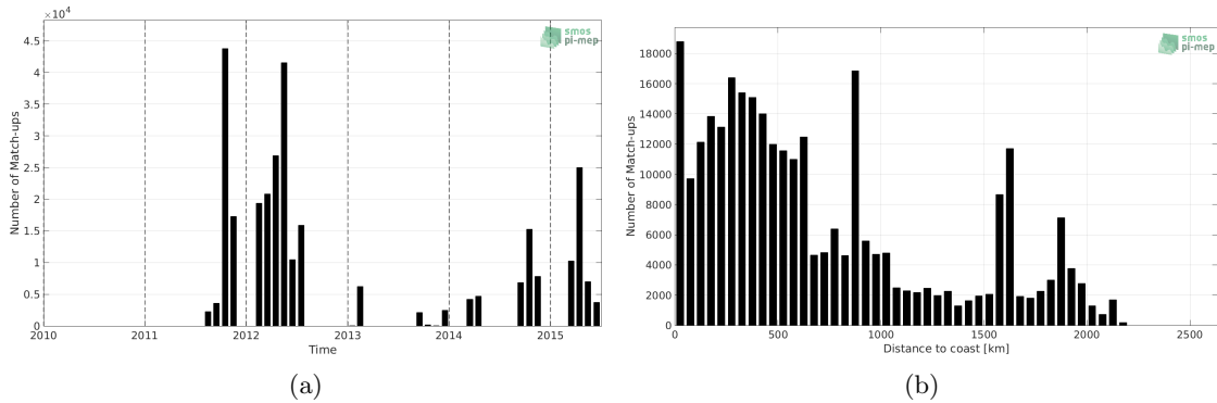
Figure 1: Number of match-ups between TSG-SAMOS and Aquarius-L4-IPRC-V5-WEEKLY SSS as a function of time (a) and as function of the distance to coast (b) over the Equatorial Ocean 10N-10S Pi-MEP region and for the full satellite product period.
