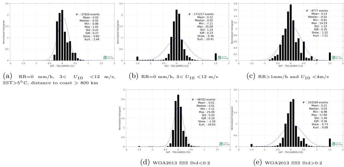
Figure 13: Normalized histogram of \Delta SSS (Aquarius-L4-IPRC-V5-WEEKLY - TSG-SAMOS) for 5 different subdatasets corresponding to: RR=0 mm/h, 3 < U_{10} < 12 m/s, SST >5^\circ\text{C} , distance to coast > 800 km (a), RR=0 mm/h, 3 < U_{10} < 12 m/s (b), RR >1 mm/h and U_{10} < 4 m/s (c), WOA2013 SSS Std <0.2 (d), WOA2013 SSS Std >0.2 (e).
