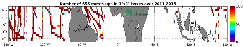
Figure 4: Number of SSS match-ups between TSG-SAMOS SSS and the Aquarius-L4-IPRC-V5-WEEKLY SSS product for the Equatorial Ocean 10N-10S Pi-MEP region over 1°x1° boxes and for the full satellite product period.
