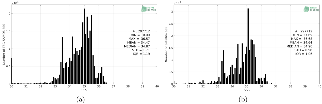
Figure 2: Histograms of SSS from TSG-SAMOS (a) and Aquarius-L4-IPRC-V5-WEEKLY (b) considering all match-up pairs per bins of 0.1 over the Equatorial Ocean 10N-10S Pi-MEP region and for the full satellite product period.
