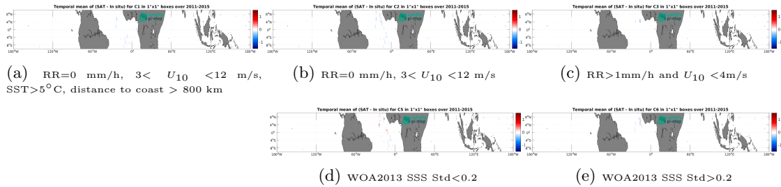
Figure 12: Temporal mean gridded over spatial boxes of size 1^\circ \times 1^\circ of \Delta SSS (Aquarius SSS L4 OI v5 - Weekly (IPRC) - TSG (Polarstern)) for 5 different subdatasets corresponding to:RR=0 mm/h, 3 < U_{10} < 12 m/s, SST >5^\circ C, distance to coast > 800 km (a), RR=0 mm/h, 3 < U_{10} < 12 m/s (b), RR >1 mm/h and U_{10} < 4 m/s (c), WOA2013 SSS Std <0.2 (d), WOA2013 SSS Std >0.2 (e).
