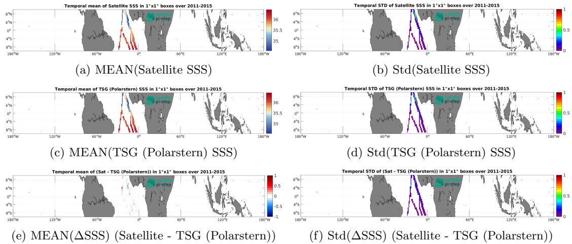
Figure 6: Temporal mean (left) and Std (right) of SSS from Aquarius SSS L4 OI v5 - Weekly (IPRC) (top), TSG (Polarstern) (middle), and of \Delta SSS (Satellite - TSG (Polarstern)). Only match-up pairs are used to generate these maps.
