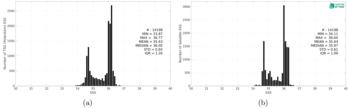
Figure 2: Histograms of SSS from TSG (Polarstern) (a) and Aquarius SSS L4 OI v5 - Weekly (IPRC) (b) considering all match-up pairs per bins of 0.1 over the Equatorial Ocean 10N-10S Pi-MEP region and for the full satellite product period.
