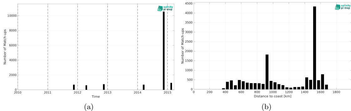
Figure 1: Number of match-ups between TSG (Polarstern) and Aquarius SSS L4 OI v5 - Weekly (IPRC) SSS as a function of time (a) and as function of the distance to coast (b) over the Equatorial Ocean 10N-10S Pi-MEP region and for the full satellite product period.
