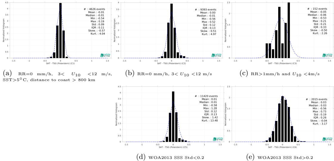
Figure 13: Normalized histogram of \Delta SSS (Aquarius SSS L4 OI v5 - Weekly (IPRC) - TSG (Polarstern)) for 5 different subdatasets corresponding to: RR=0 mm/h, 3 < U_{10} < 12 m/s, SST >5^\circ C, distance to coast > 800 km (a), RR=0 mm/h, 3 < U_{10} < 12 m/s (b), RR >1 mm/h and U_{10} < 4 m/s (c), WOA2013 SSS Std <0.2 (d), WOA2013 SSS Std >0.2 (e).
