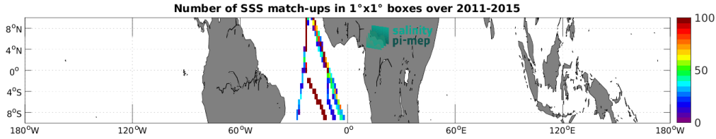
Figure 4: Number of SSS match-ups between TSG (Polarstern) SSS and the Aquarius SSS L4 OI v5 - Weekly (IPRC) SSS product for the Equatorial Ocean 10N-10S Pi-MEP region over 1^\circ \times 1^\circ boxes and for the full satellite product period.
