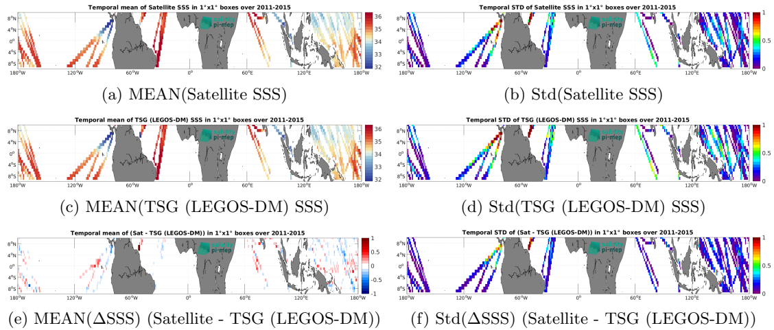
Figure 7: Temporal mean (left) and Std (right) of SSS from Aquarius SSS L4 OI v5 - Weekly (IPRC) (top), TSG (LEGOS-DM) (middle), and of \Delta SSS (Satellite - TSG (LEGOS-DM)). Only match-up pairs are used to generate these maps.
