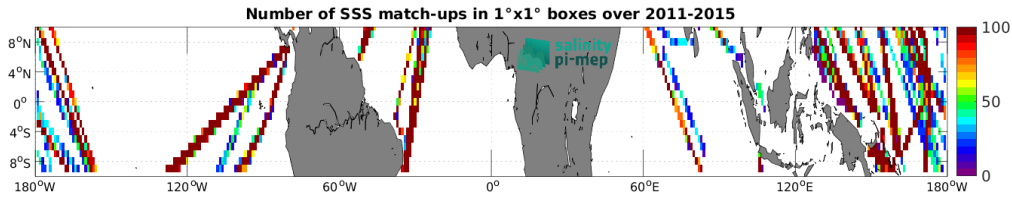
Figure 5: Number of SSS match-ups between TSG (LEGOS-DM) SSS and the Aquarius SSS L4 OI v5 - Weekly (IPRC) SSS product for the Equatorial Ocean 10N-10S Pi-MEP region over 1^\circ \times 1^\circ boxes and for the full satellite product period.
