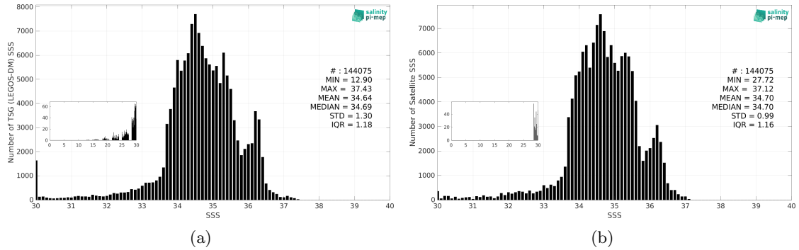
Figure 3: Histograms of SSS from TSG (LEGOS-DM) (a) and Aquarius SSS L4 OI v5 - Weekly (IPRC) (b) considering all match-up pairs per bins of 0.1 over the Equatorial Ocean 10N-10S Pi-MEP region and for the full satellite product period.
