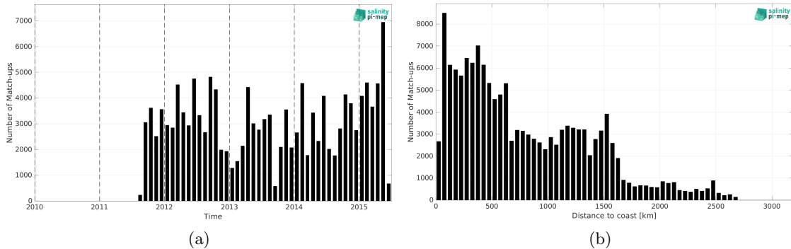
Figure 2: Number of match-ups between TSG (LEGOS-DM) and Aquarius SSS L4 OI v5 - Weekly (IPRC) SSS as a function of time (a) and as function of the distance to coast (b) over the Equatorial Ocean 10N-10S Pi-MEP region and for the full satellite product period.
