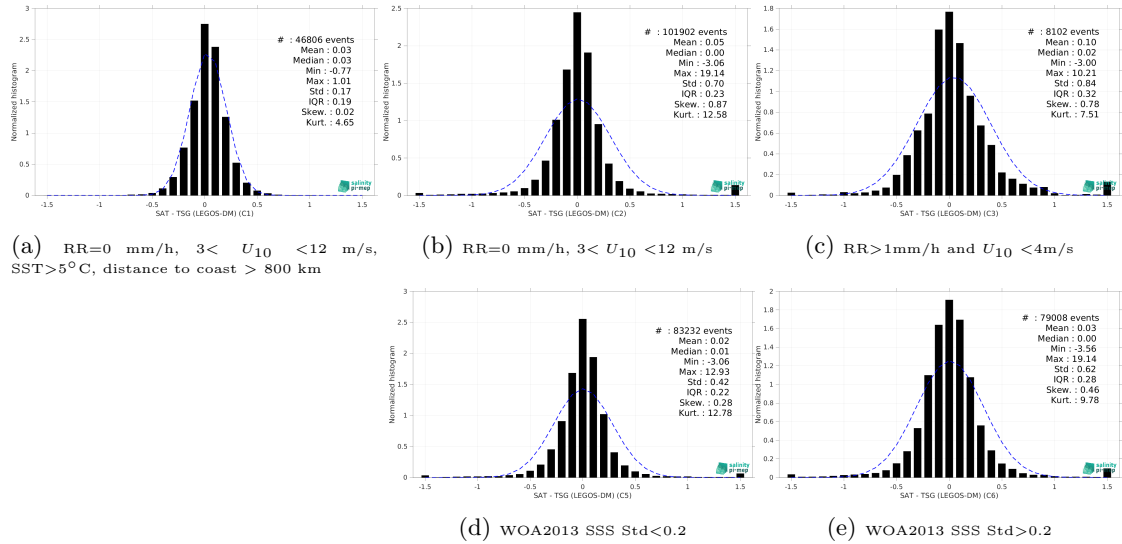
Figure 13: Normalized histogram of \Delta SSS (Aquarius SSS L4 OI v5 - Weekly (IPRC) - TSG (LEGOS-DM)) for 5 different subdatasets corresponding to: RR=0 mm/h, 3 < U_{10} < 12 m/s, SST > 5^\circ C , distance to coast > 800 km (a), RR=0 mm/h, 3 < U_{10} < 12 m/s (b), RR > 1 mm/h and U_{10} < 4 m/s (c), WOA2013 SSS Std <0.2 (d), WOA2013 SSS Std >0.2 (e).
