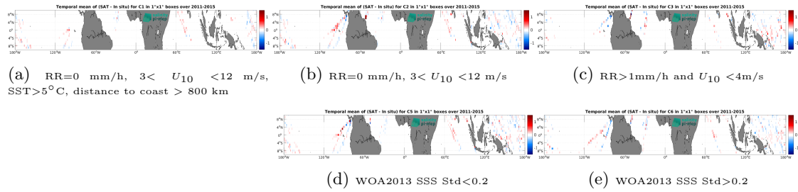
Figure 12: Temporal mean gridded over spatial boxes of size 1^\circ \times 1^\circ of \Delta SSS (Aquarius SSS L4 OI v5 - Weekly (IPRC) - TSG (LEGOS-DM)) for 5 different subdatasets corresponding to: RR=0 mm/h, 3 < U_{10} < 12 m/s, SST > 5^\circ C , distance to coast > 800 km (a), RR=0 mm/h, 3 < U_{10} < 12 m/s (b), RR > 1 mm/h and U_{10} < 4 m/s (c), WOA2013 SSS Std <0.2 (d), WOA2013 SSS Std >0.2 (e).
