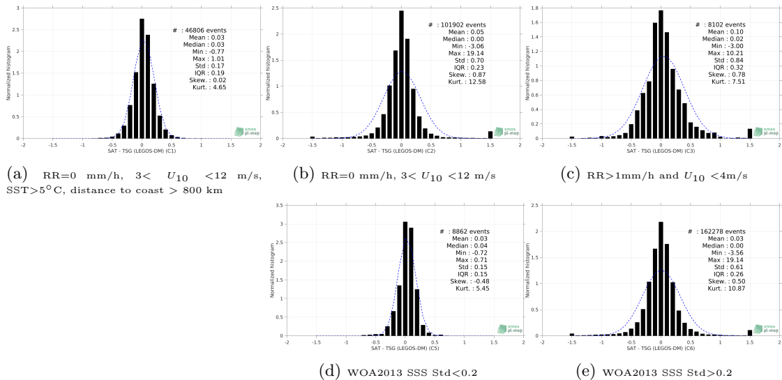
Figure 13: Normalized histogram of ΔSSS (Aquarius SSS L4 OI v5 - Weekly (IPRC) - TSG (LEGOS-DM)) for 5 different subdatasets corresponding to: RR=0 mm/h, 3 < U_{10} < 12 m/s, SST>5°C, distance to coast > 800 km (a), RR=0 mm/h, 3 < U_{10} < 12 m/s (b), RR>1mm/h and U_{10} < 4m/s (c), WOA2013 SSS Std<0.2 (d), WOA2013 SSS Std>0.2 (e).
