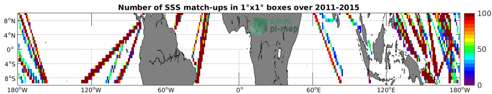
Figure 4: Number of SSS match-ups between TSG (LEGOS-DM) SSS and the Aquarius SSS L4 OI v5 - Weekly (IPRC) SSS product for the Equatorial Ocean 10N-10S Pi-MEP region over 1°x1° boxes and for the full satellite product period.
