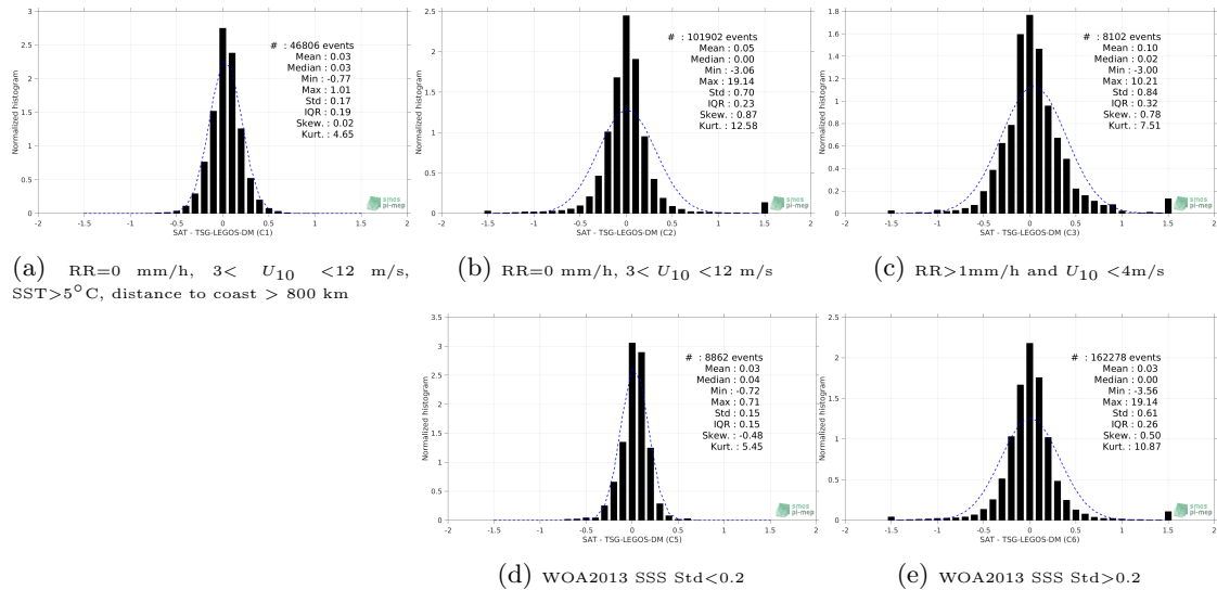
Figure 13: Normalized histogram of \Delta SSS (Aquarius-L4-IPRC-V5-WEEKLY - TSG-LEGOS-DM) for 5 different subdatasets corresponding to: RR=0 mm/h, 3 < U_{10} < 12 m/s, SST >5^\circ\text{C} , distance to coast > 800 km (a), RR=0 mm/h, 3 < U_{10} < 12 m/s (b), RR >1 mm/h and U_{10} < 4 m/s (c), WOA2013 SSS Std <0.2 (d), WOA2013 SSS Std >0.2 (e).
