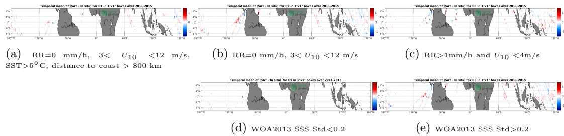
Figure 12: Temporal mean gridded over spatial boxes of size 1^\circ \times 1^\circ of \Delta SSS (Aquarius-L4-IPRC-V5-WEEKLY - TSG-LEGOS-DM) for 5 different subdatasets corresponding to:RR=0 mm/h, 3 < U_{10} < 12 m/s, SST >5^\circ\text{C} , distance to coast > 800 km (a), RR=0 mm/h, 3 < U_{10} < 12 m/s (b), RR >1 mm/h and U_{10} < 4 m/s (c), WOA2013 SSS Std <0.2 (d), WOA2013 SSS Std >0.2 (e).
