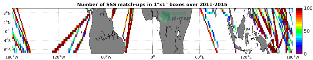
Figure 4: Number of SSS match-ups between TSG-LEGOS-DM SSS and the Aquarius-L4-IPRC-V5-WEEKLY SSS product for the Equatorial Ocean 10N-10S Pi-MEP region over 1^\circ \times 1^\circ boxes and for the full satellite product period.
