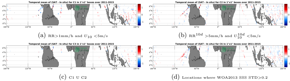
Figure 12: Temporal mean gridded over spatial boxes of size 1^\circ \times 1^\circ of \Delta SSS (Aquarius-L4-IPRC-V5-WEEKLY - TSG-LEGOS-DM) for 4 different subdatasets corresponding to: RR > 1\text{mm/h} and U_{10} < 5\text{m/s} (a), RR^{10d} > 5\text{mm/h} and U_{10}^{10d} < 5\text{m/s} (b), C1 U C2 (c), Locations where WOA2013 SSS STD > 0.2 (d).
