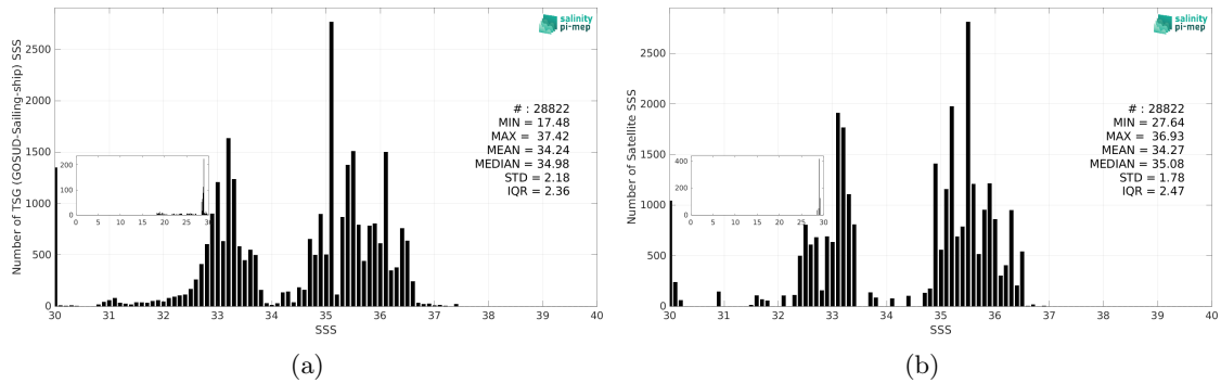
Figure 3: Histograms of SSS from TSG (GOSUD-Sailing-ship) (a) and Aquarius SSS L4 OI v5 - Weekly (IPRC) (b) considering all match-up pairs per bins of 0.1 over the Equatorial Ocean 10N-10S Pi-MEP region and for the full satellite product period.
