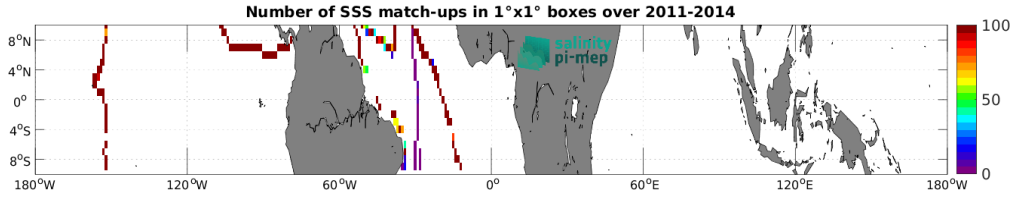
Figure 5: Number of SSS match-ups between TSG (GOSUD-Sailing-ship) SSS and the Aquarius SSS L4 OI v5 - Weekly (IPRC) SSS product for the Equatorial Ocean 10N-10S Pi-MEP region over 1^\circ \times 1^\circ boxes and for the full satellite product period.
