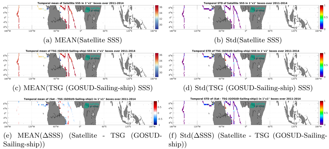
Figure 7: Temporal mean (left) and Std (right) of SSS from Aquarius SSS L4 OI v5 - Weekly (IPRC) (top), TSG (GOSUD-Sailing-ship) (middle), and of \Delta SSS (Satellite - TSG (GOSUD-Sailing-ship)). Only match-up pairs are used to generate these maps.
