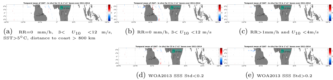
Figure 14: Temporal mean gridded over spatial boxes of size 1^\circ \times 1^\circ of \Delta SSS (Aquarius SSS L4 OI v5 - Weekly (IPRC) - TSG (GOSUD-Sailing-ship)) for 5 different subdatasets corresponding to: RR=0 mm/h, 3 < U_{10} < 12 m/s, SST>5°C, distance to coast > 800 km (a), RR=0 mm/h, 3 < U_{10} < 12 m/s (b), RR>1mm/h and U_{10} < 4 m/s (c), WOA2013 SSS Std<0.2 (d), WOA2013 SSS Std>0.2 (e).
