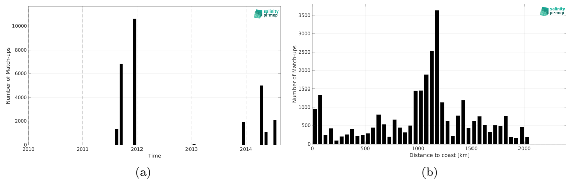
Figure 2: Number of match-ups between TSG (GOSUD-Sailing-ship) and Aquarius SSS L4 OI v5 - Weekly (IPRC) SSS as a function of time (a) and as function of the distance to coast (b) over the Equatorial Ocean 10N-10S Pi-MEP region and for the full satellite product period.
