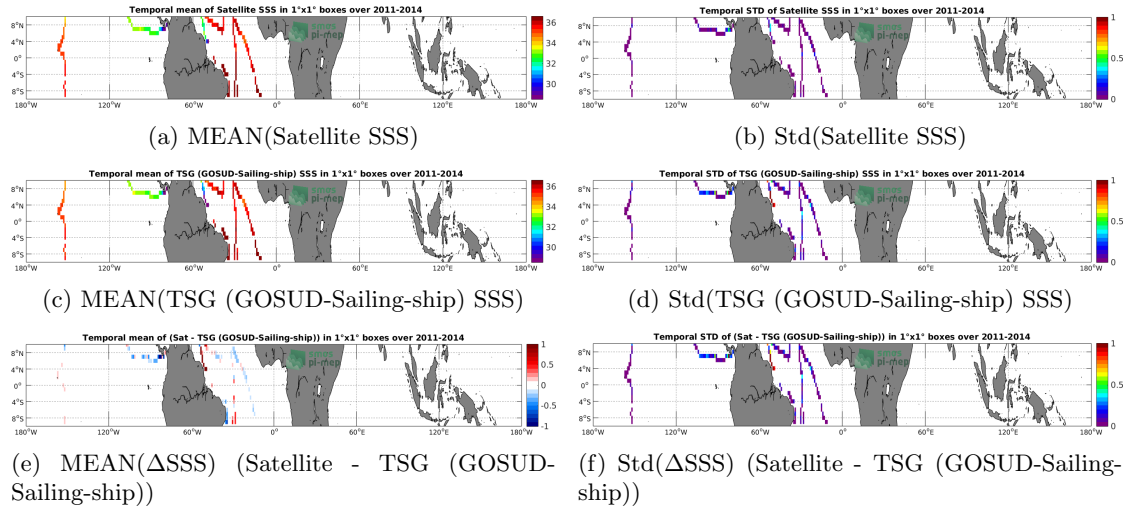
Figure 6: Temporal mean (left) and Std (right) of SSS from Aquarius SSS L4 OI v5 - Weekly (IPRC) (top), TSG (GOSUD-Sailing-ship) (middle), and of \Delta SSS (Satellite - TSG (GOSUD-Sailing-ship)). Only match-up pairs are used to generate these maps.
