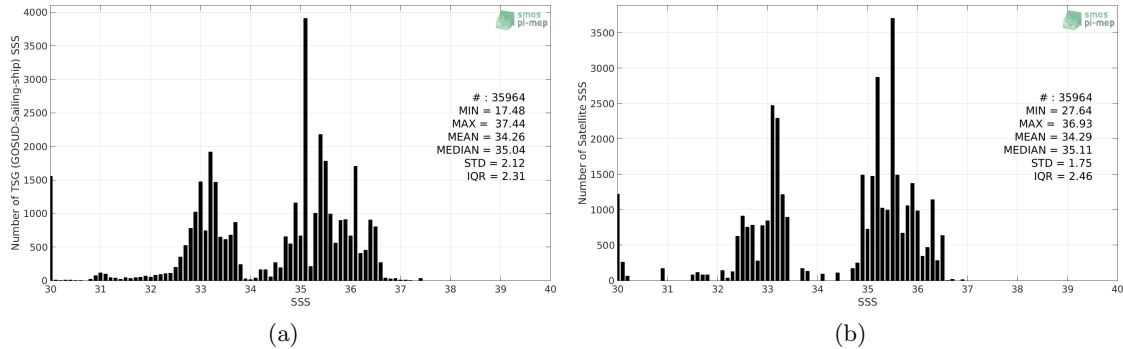
Figure 2: Histograms of SSS from TSG (GOSUD-Sailing-ship) (a) and Aquarius SSS L4 OI v5 - Weekly (IPRC) (b) considering all match-up pairs per bins of 0.1 over the Equatorial Ocean 10N-10S Pi-MEP region and for the full satellite product period.
