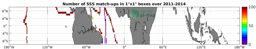
Figure 4: Number of SSS match-ups between TSG (GOSUD-Sailing-ship) SSS and the Aquarius SSS L4 OI v5 - Weekly (IPRC) SSS product for the Equatorial Ocean 10N-10S Pi-MEP region over 1^\circ \times 1^\circ boxes and for the full satellite product period.
