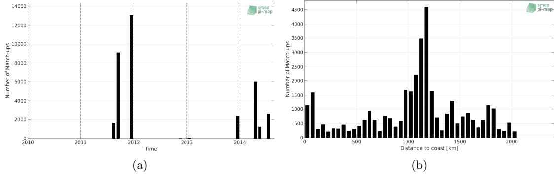
Figure 1: Number of match-ups between TSG (GOSUD-Sailing-ship) and Aquarius SSS L4 OI v5 - Weekly (IPRC) SSS as a function of time (a) and as function of the distance to coast (b) over the Equatorial Ocean 10N-10S Pi-MEP region and for the full satellite product period.
