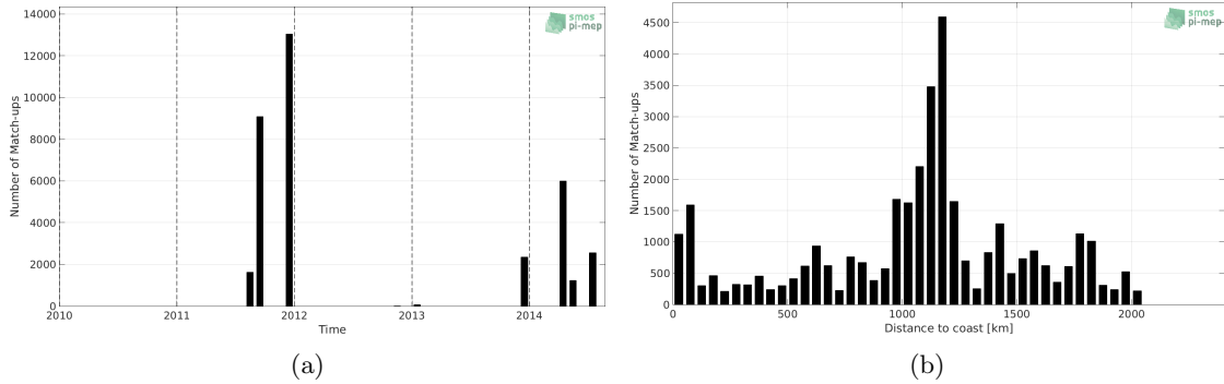
Figure 1: Number of match-ups between TSG-GOSUD-Sailing-ship and Aquarius-L4-IPRC-V5-WEEKLY SSS as a function of time (a) and as function of the distance to coast (b) over the Equatorial Ocean 10N-10S Pi-MEP region and for the full satellite product period.
