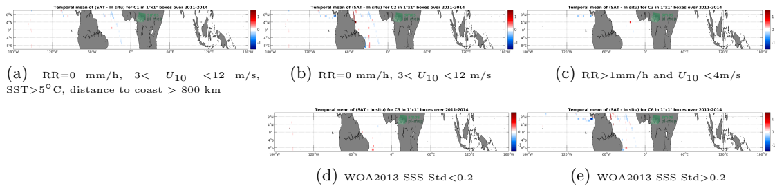
Figure 12: Temporal mean gridded over spatial boxes of size 1^\circ \times 1^\circ of \Delta SSS (Aquarius-L4-IPRC-V5-WEEKLY - TSG-GOSUD-Sailing-ship) for 5 different subdatasets corresponding to: RR=0 mm/h, 3 < U_{10} < 12 m/s, SST>5°C, distance to coast > 800 km (a), RR=0 mm/h, 3 < U_{10} < 12 m/s (b), RR>1mm/h and U_{10} < 4 m/s (c), WOA2013 SSS Std<0.2 (d), WOA2013 SSS Std>0.2 (e).
