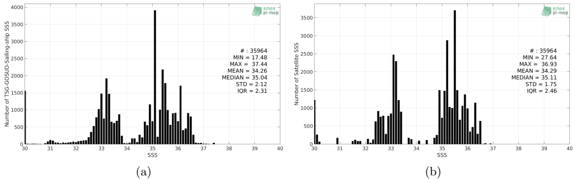
Figure 2: Histograms of SSS from TSG-GOSUD-Sailing-ship (a) and Aquarius-L4-IPRC-V5-WEEKLY (b) considering all match-up pairs per bins of 0.1 over the Equatorial Ocean 10N-10S Pi-MEP region and for the full satellite product period.
