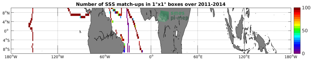
Figure 4: Number of SSS match-ups between TSG-GOSUD-Sailing-ship SSS and the Aquarius-L4-IPRC-V5-WEEKLY SSS product for the Equatorial Ocean 10N-10S Pi-MEP region over 1°x1° boxes and for the full satellite product period.
