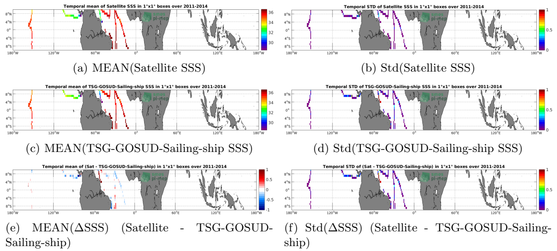
Figure 6: Temporal mean (left) and Std (right) of SSS from Aquarius-L4-IPRC-V5-WEEKLY (top), TSG-GOSUD-Sailing-ship (middle), and of \Delta SSS (Satellite - TSG-GOSUD-Sailing-ship). Only match-up pairs are used to generate these maps.
