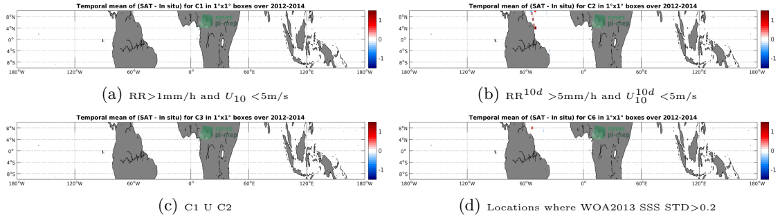
Figure 12: Temporal mean gridded over spatial boxes of size 1^\circ \times 1^\circ of \Delta SSS (Aquarius-L4-IPRC-V5-WEEKLY - TSG-GOSUD-Sailing-ship) for 4 different subdatasets corresponding to: RR > 1\text{mm/h} and U_{10} < 5\text{m/s} (a), RR^{10d} > 5\text{mm/h} and U_{10}^{10d} < 5\text{m/s} (b), C1 U C2 (c), Locations where WOA2013 SSS STD > 0.2 (d).
