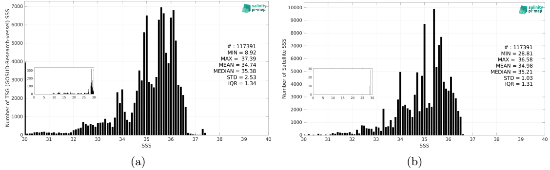
Figure 3: Histograms of SSS from TSG (GOSUD-Research-vessel) (a) and Aquarius SSS L4 OI v5 - Weekly (IPRC) (b) considering all match-up pairs per bins of 0.1 over the Equatorial Ocean 10N-10S Pi-MEP region and for the full satellite product period.
