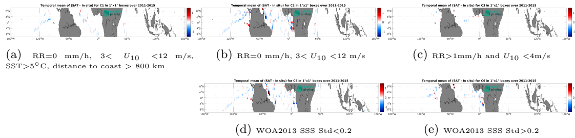
Figure 14: Temporal mean gridded over spatial boxes of size 1^\circ \times 1^\circ of \Delta SSS (Aquarius SSS L4 OI v5 - Weekly (IPRC) - TSG (GOSUD-Research-vessel)) for 5 different subdatasets corresponding to: RR=0 mm/h, 3 < U_{10} < 12 m/s, SST>5°C, distance to coast > 800 km (a), RR=0 mm/h, 3 < U_{10} < 12 m/s (b), RR>1mm/h and U_{10} < 4 m/s (c), WOA2013 SSS Std<0.2 (d), WOA2013 SSS Std>0.2 (e).
