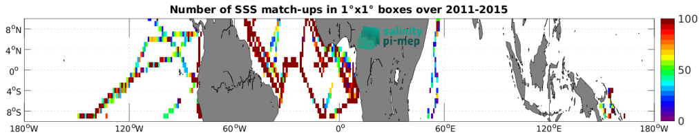
Figure 5: Number of SSS match-ups between TSG (GOSUD-Research-vessel) SSS and the Aquarius SSS L4 OI v5 - Weekly (IPRC) SSS product for the Equatorial Ocean 10N-10S Pi-MEP region over 1^\circ \times 1^\circ boxes and for the full satellite product period.
