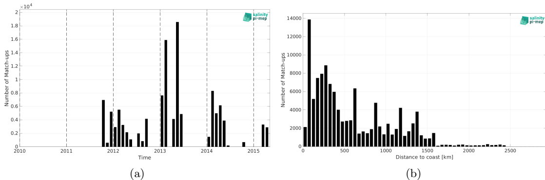
Figure 2: Number of match-ups between TSG (GOSUD-Research-vessel) and Aquarius SSS L4 OI v5 - Weekly (IPRC) SSS as a function of time (a) and as function of the distance to coast (b) over the Equatorial Ocean 10N-10S Pi-MEP region and for the full satellite product period.
