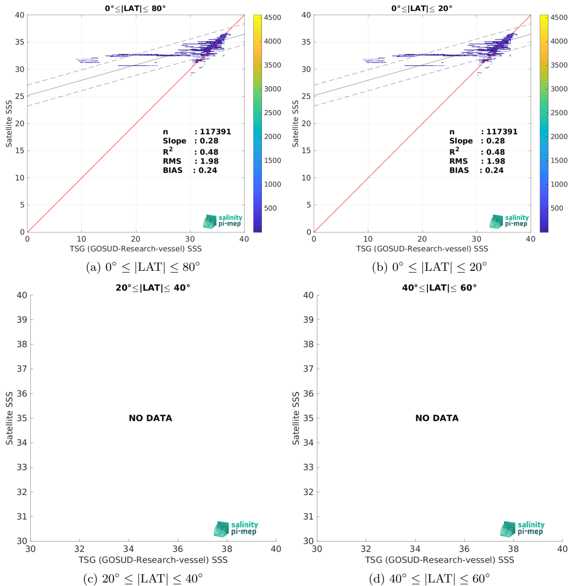
Figure 10: Contour maps of the concentration of Aquarius SSS L4 OI v5 - Weekly (IPRC) SSS (y-axis) versus TSG (GOSUD-Research-vessel) SSS (x-axis) at match-up pairs for different latitude bands. For each plot, the red line shows x=y . The black thin and dashed lines indicate a linear fit through the data cloud and the \pm 95\% confidence levels, respectively. The number match-up pairs n , the slope and R^2 coefficient of the linear fit, the root mean square (RMS) and the mean bias between satellite and in situ data are indicated for each latitude band in each plots.
