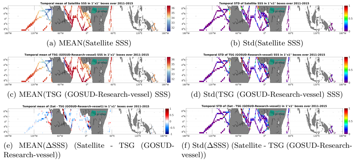
Figure 7: Temporal mean (left) and Std (right) of SSS from Aquarius SSS L4 OI v5 - Weekly (IPRC) (top), TSG (GOSUD-Research-vessel) (middle), and of \Delta SSS (Satellite - TSG (GOSUD-Research-vessel)). Only match-up pairs are used to generate these maps.
