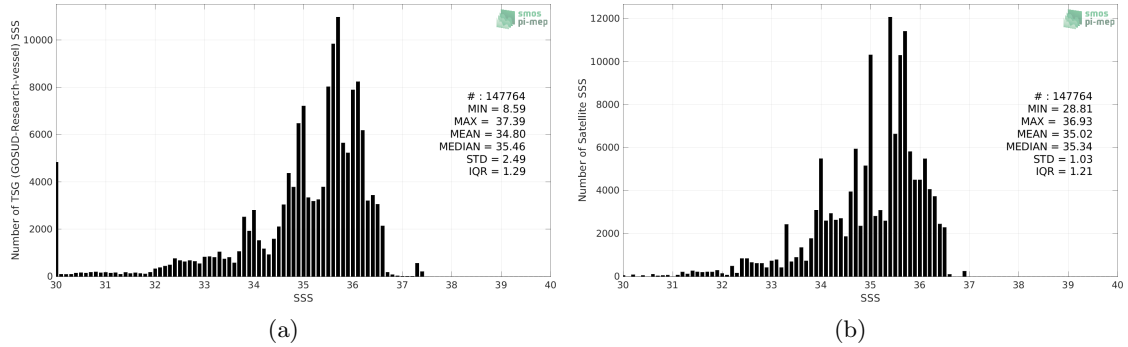
Figure 2: Histograms of SSS from TSG (GOSUD-Research-vessel) (a) and Aquarius SSS L4 OI v5 - Weekly (IPRC) (b) considering all match-up pairs per bins of 0.1 over the Equatorial Ocean 10N-10S Pi-MEP region and for the full satellite product period.
