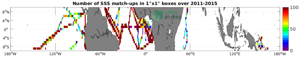
Figure 4: Number of SSS match-ups between TSG (GOSUD-Research-vessel) SSS and the Aquarius SSS L4 OI v5 - Weekly (IPRC) SSS product for the Equatorial Ocean 10N-10S Pi-MEP region over 1^\circ \times 1^\circ boxes and for the full satellite product period.
