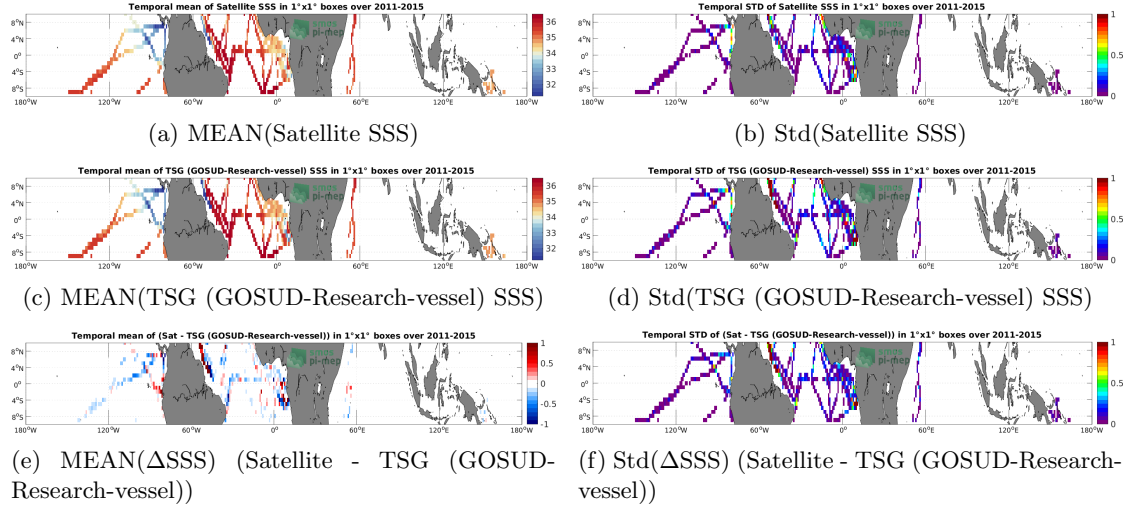
Figure 6: Temporal mean (left) and Std (right) of SSS from Aquarius SSS L4 OI v5 - Weekly (IPRC) (top), TSG (GOSUD-Research-vessel) (middle), and of \Delta SSS (Satellite - TSG (GOSUD-Research-vessel)). Only match-up pairs are used to generate these maps.
