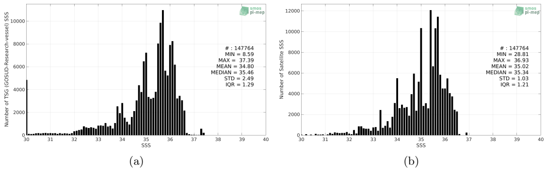
Figure 2: Histograms of SSS from TSG (GOSUD-Research-vessel) (a) and Aquarius SSS L4 OI v5 - Weekly (IPRC) (b) considering all match-up pairs per bins of 0.1 over the Equatorial Ocean 10N-10S Pi-MEP region and for the full satellite product period.
