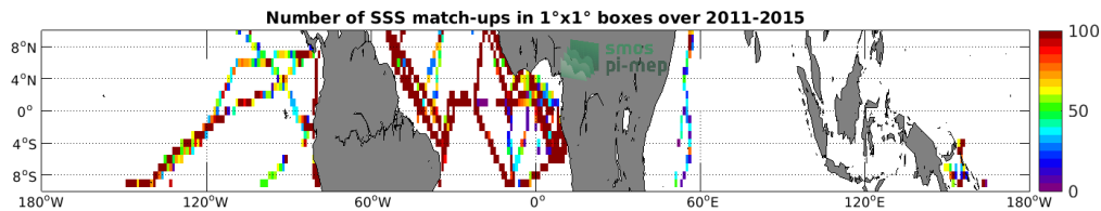
Figure 4: Number of SSS match-ups between TSG (GOSUD-Research-vessel) SSS and the Aquarius SSS L4 OI v5 - Weekly (IPRC) SSS product for the Equatorial Ocean 10N-10S Pi-MEP region over 1°x1° boxes and for the full satellite product period.
