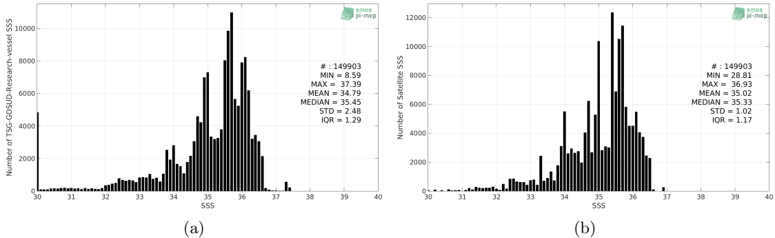
Figure 2: Histograms of SSS from TSG-GOSUD-Research-vessel (a) and Aquarius-L4-IPRC-V5-WEEKLY (b) considering all match-up pairs per bins of 0.1 over the Equatorial Ocean 10N-10S Pi-MEP region and for the full satellite product period.
