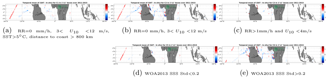
Figure 12: Temporal mean gridded over spatial boxes of size 1^\circ \times 1^\circ of \Delta SSS (Aquarius-L4-IPRC-V5-WEEKLY - TSG-GOSUD-Research-vessel) for 5 different subdatasets corresponding to: RR=0 mm/h, 3 < U_{10} < 12 m/s, SST>5°C, distance to coast > 800 km (a), RR=0 mm/h, 3 < U_{10} < 12 m/s (b), RR>1mm/h and U_{10} < 4 m/s (c), WOA2013 SSS Std<0.2 (d), WOA2013 SSS Std>0.2 (e).
