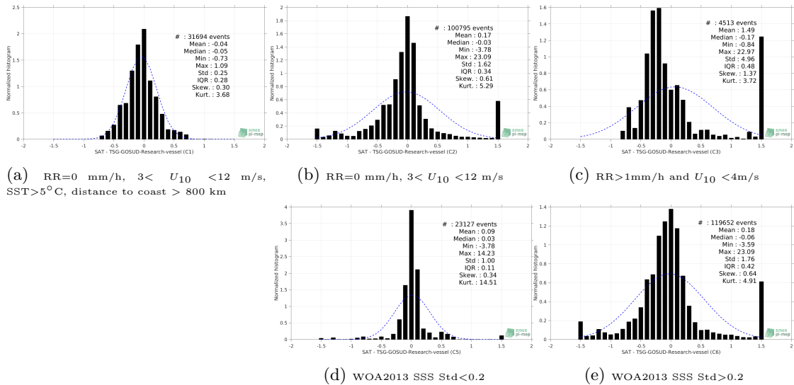
Figure 13: Normalized histogram of \Delta SSS (Aquarius-L4-IPRC-V5-WEEKLY - TSG-GOSUD-Research-vessel) for 5 different subdatasets corresponding to: RR=0 mm/h, 3 < U_{10} < 12 m/s, SST >5^\circ\text{C} , distance to coast > 800 km (a), RR=0 mm/h, 3 < U_{10} < 12 m/s (b), RR >1 mm/h and U_{10} < 4 m/s (c), WOA2013 SSS Std <0.2 (d), WOA2013 SSS Std >0.2 (e).
