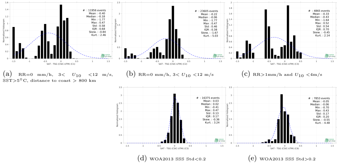
Figure 13: Normalized histogram of \Delta SSS (Aquarius SSS L4 OI v5 - Weekly (IPRC)) - TSG (CSIC-UTM) for 5 different subdatasets corresponding to: RR=0 mm/h, 3 < U_{10} < 12 m/s, SST > 5^\circ C , distance to coast > 800 km (a), RR=0 mm/h, 3 < U_{10} < 12 m/s (b), RR>1mm/h and U_{10} < 4 m/s (c), WOA2013 SSS Std<0.2 (d), WOA2013 SSS Std>0.2 (e).
